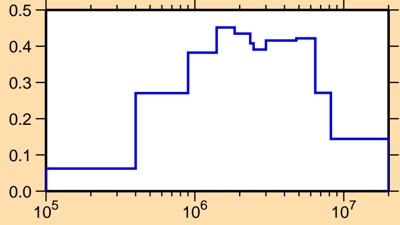
\sigma vs. E for ^{241}\text{Es}(n,\text{inel.})
