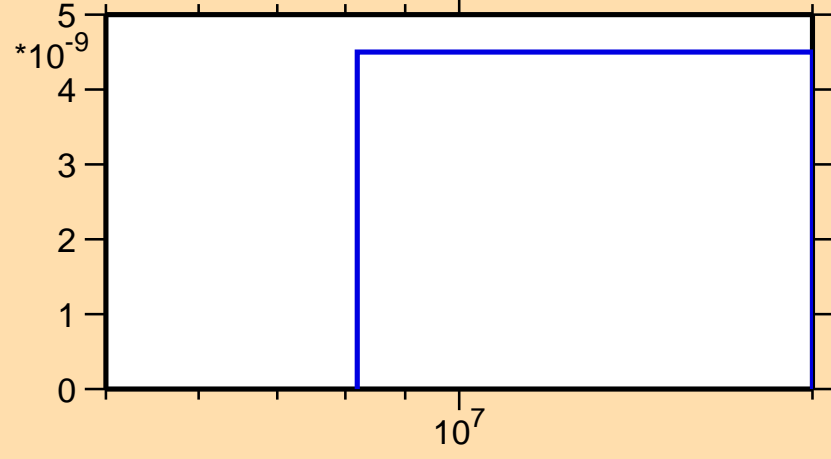
\sigma vs. E for ^{241}\text{Es}(n,2np)
