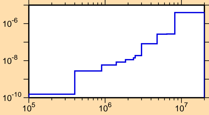
\sigma vs. E for ^{241}\text{Es}(n,n\alpha)
