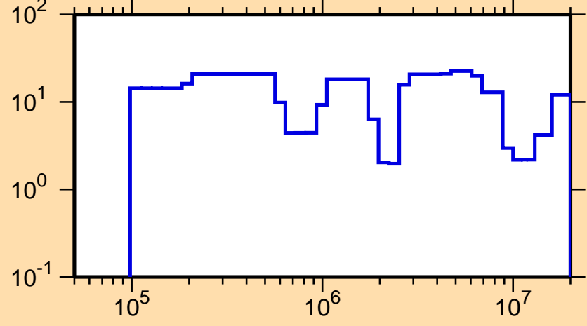
\Delta\sigma/\sigma vs. E for ^{242}\text{Es}(n,\text{el.})
