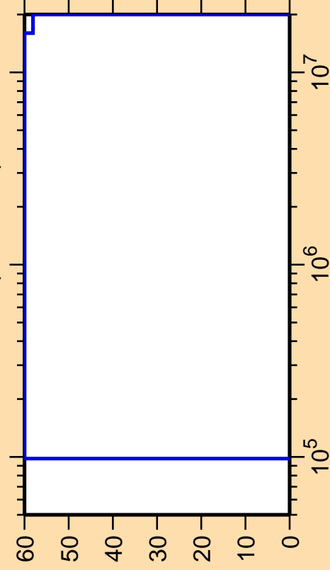
\Delta\sigma/\sigma vs. E for ^{242}\text{Es}(n, ncont.)
