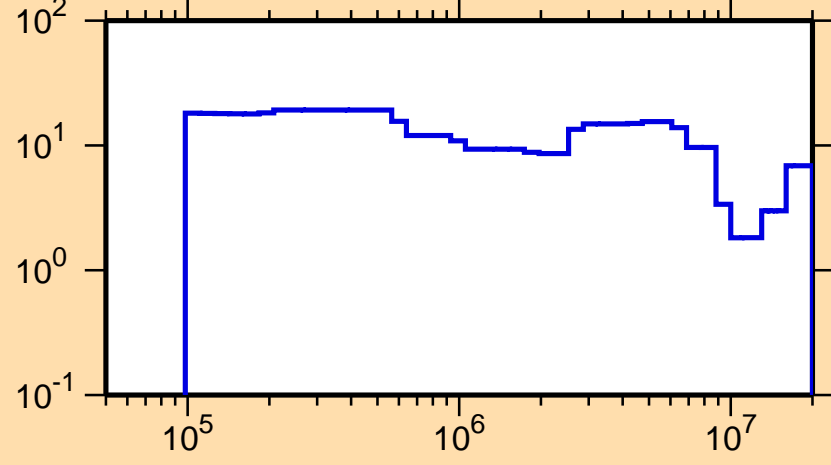
\Delta\sigma/\sigma vs. E for ^{242}\text{Es}(n, \text{tot.})
