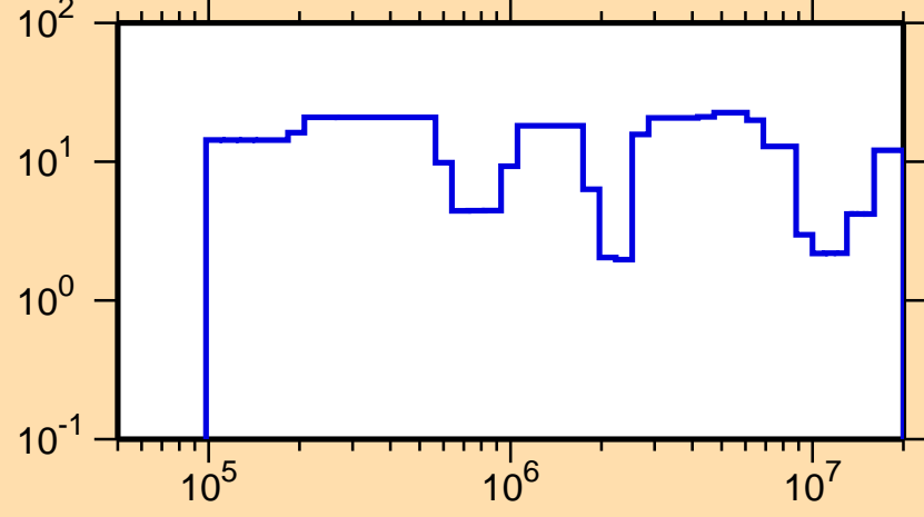
\Delta\sigma/\sigma vs. E for ^{242}\text{Es}(n, el.)
