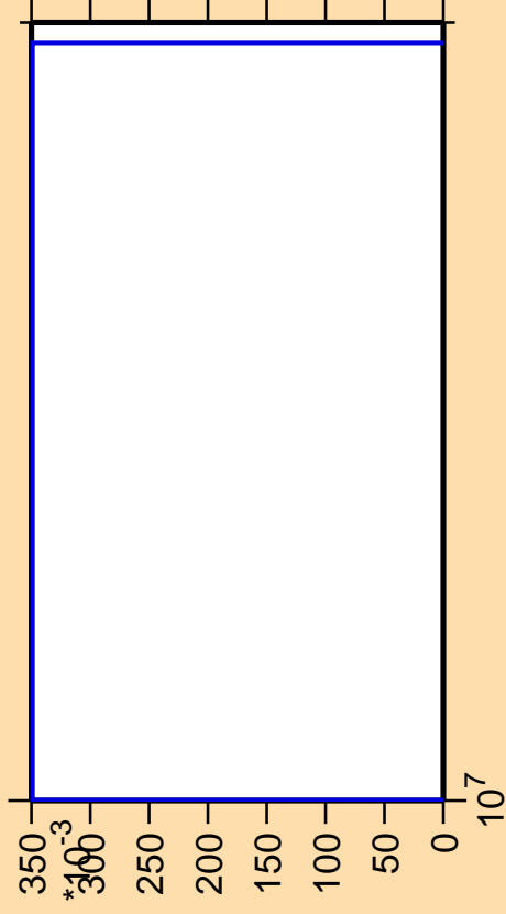
\Delta\sigma/\sigma vs. E for ^{242}\text{Es}(n,3n\alpha)
