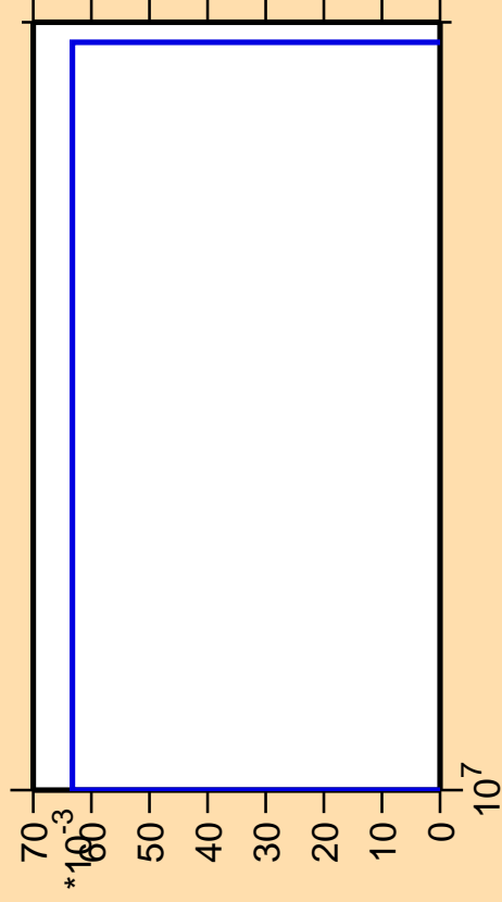
\Delta\sigma/\sigma vs. E for ^{242}\text{Es}(n,\text{pd})
