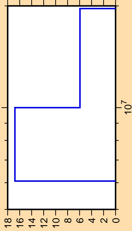
\Delta\sigma/\sigma vs. E for ^{242}\text{Es}(n,f)
