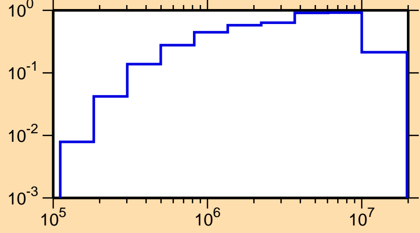
\sigma vs. E for ^{242}\text{Es}(n,\text{inel.})
