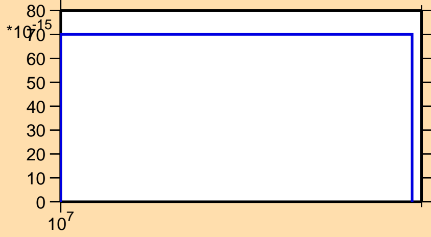
\sigma vs. E for ^{242}\text{Es}(n,\text{pd})
