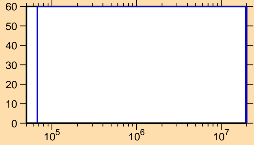
\Delta\sigma/\sigma vs. E for ^{242}\text{Es}(n,inel.)
