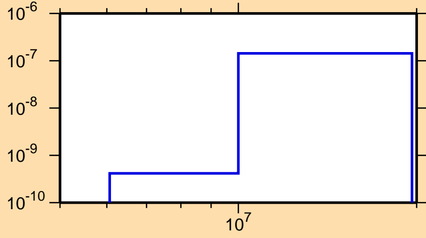
\sigma vs. E for ^{242}\text{Es}(n,2n\alpha)
