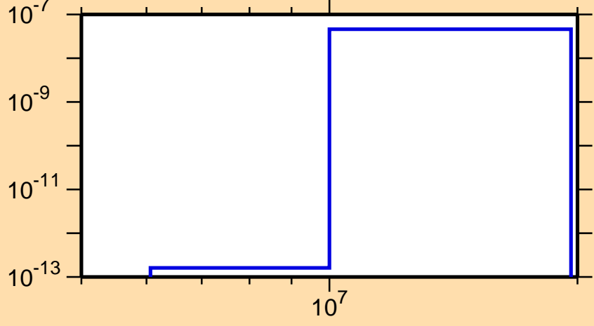
\sigma vs. E for ^{242}\text{Es}(n,\text{He3})
