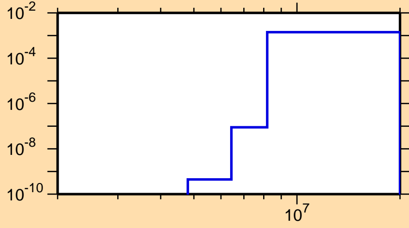
\sigma vs. E for ^{242}\text{Es}(n,d)
