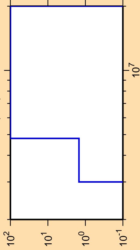
\Delta\sigma/\sigma vs. E for ^{242}\text{Es}(n,d)
