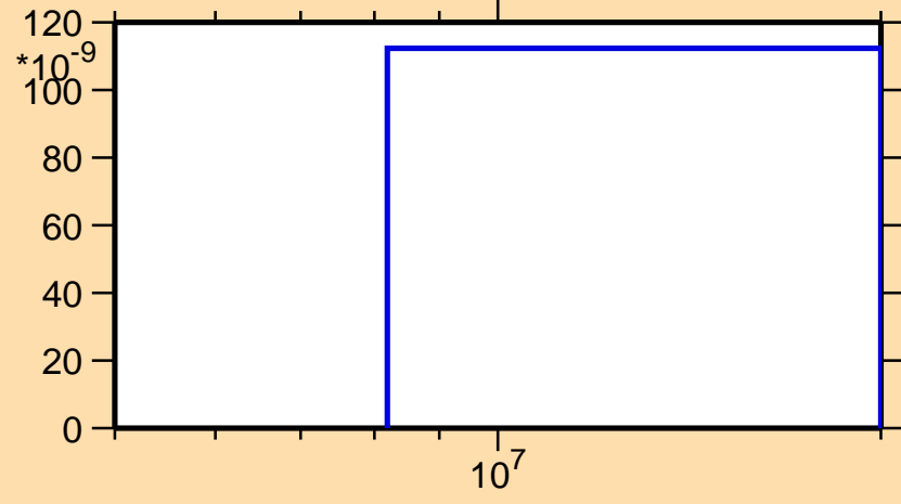
\sigma vs. E for ^{242}\text{Es}(n,nd)
