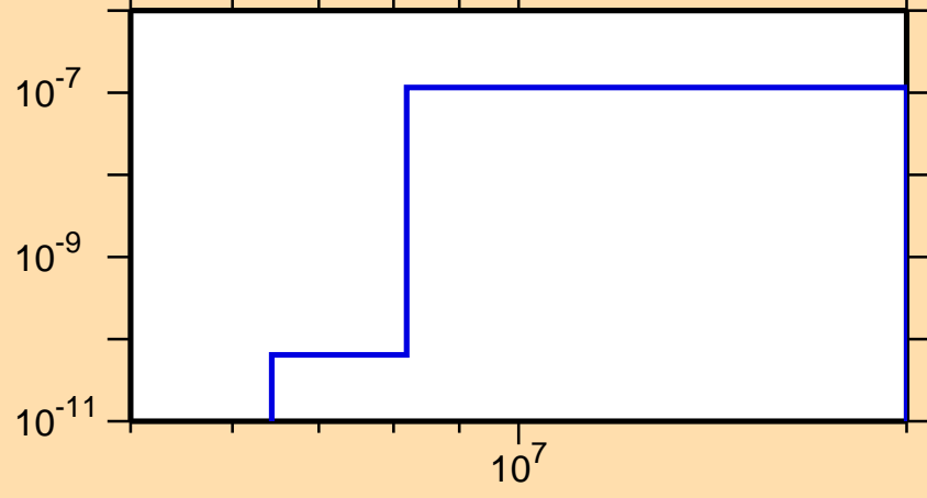
\sigma vs. E for ^{242}\text{Es}(n,2n\alpha)
