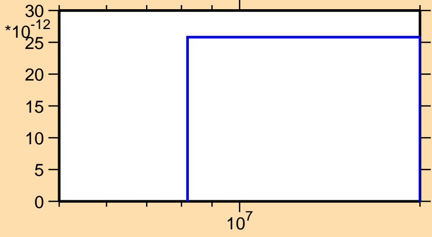
\sigma vs. E for ^{243}\text{Es}(\text{mt } 45)
