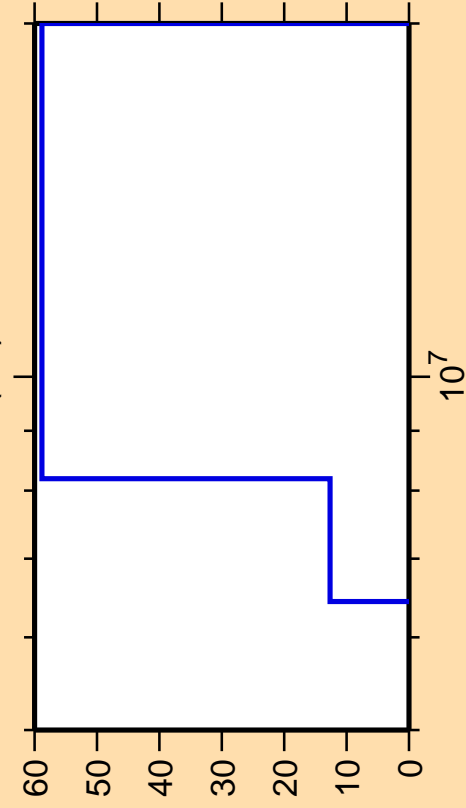
\Delta\sigma/\sigma vs. E for ^{243}\text{Es}(n,t)
