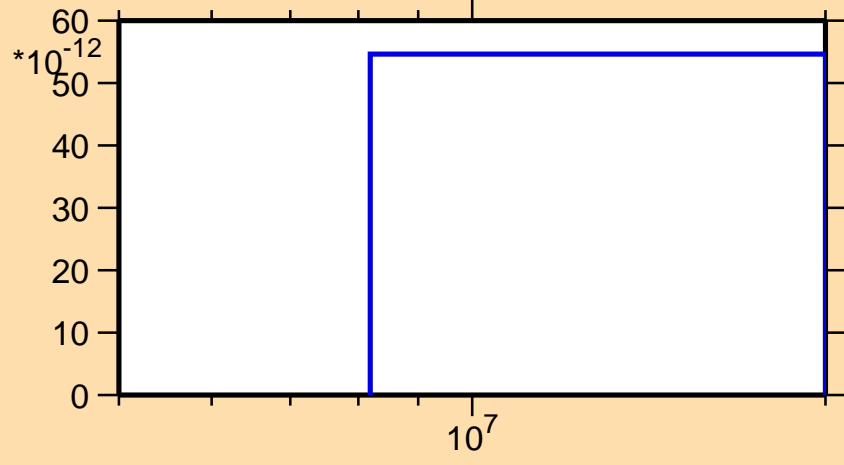
\sigma vs. E for ^{243}\text{Es}(\text{mt117})
