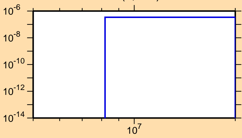
\sigma vs. E for ^{243}\text{Es}(n,2n\alpha)
