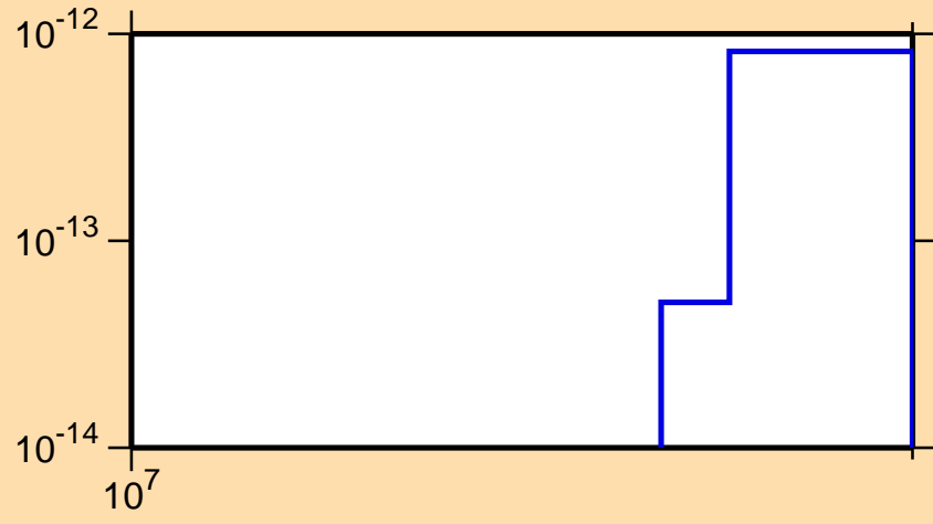
\sigma vs. E for ^{244}\text{Es}(n,\text{pd})
