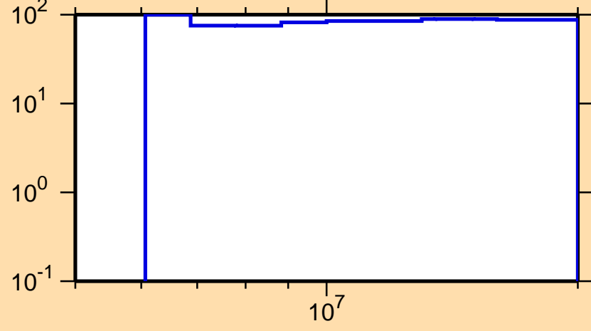
\Delta\sigma/\sigma vs. E for ^{244}\text{Es}(n,2n)
