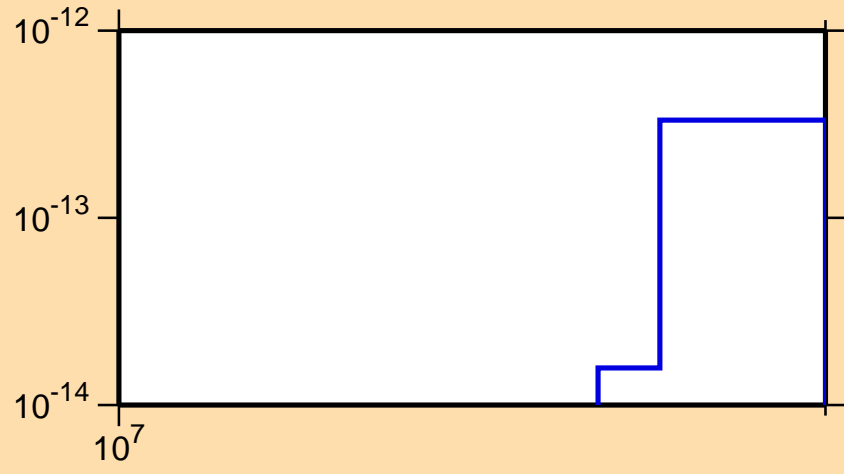
\sigma vs. E for ^{244}\text{Es}(n,pt)
