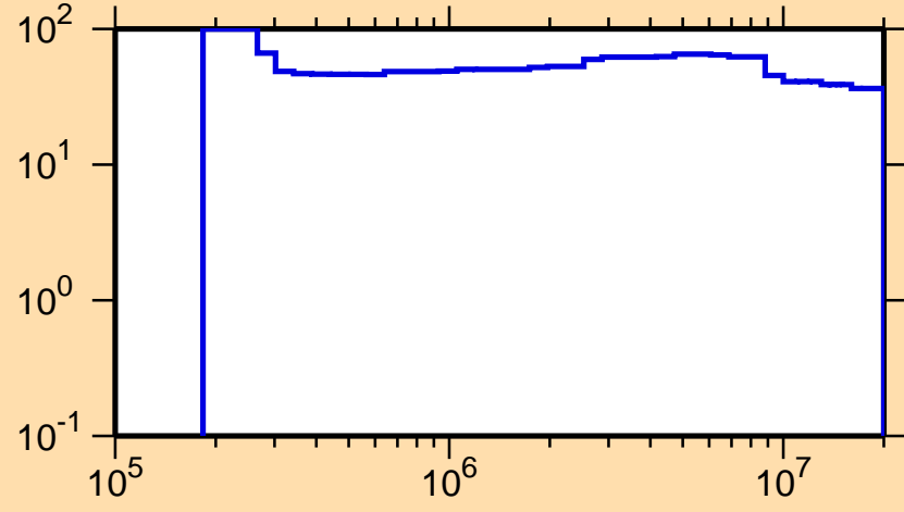
\Delta\sigma/\sigma vs. E for ^{244}\text{Es}(n,\text{inel.})
