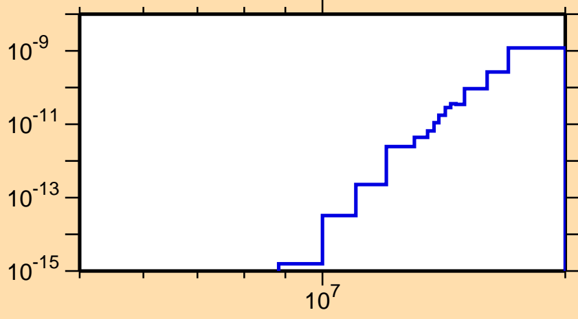
\sigma vs. E for ^{244}\text{Es} (mt 45)
