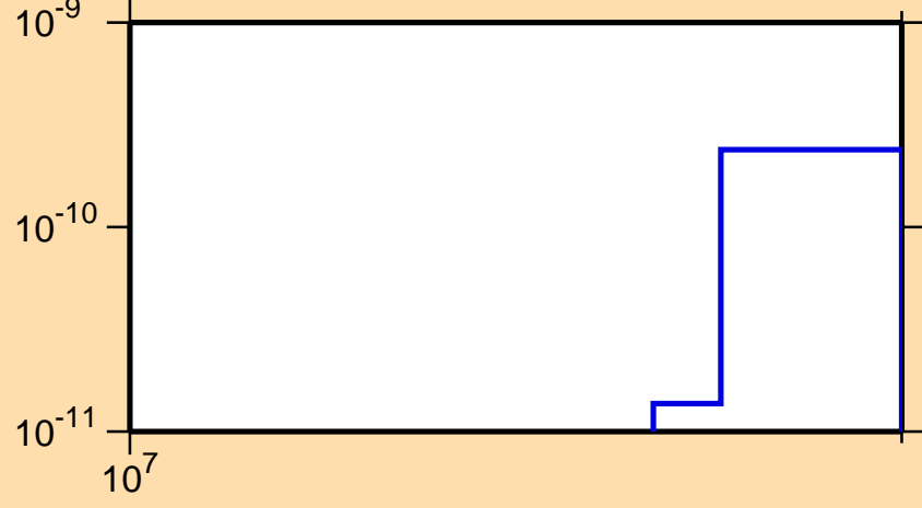
\sigma vs. E for ^{244}\text{Es}(n,3n\alpha)
