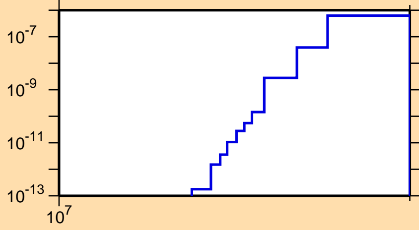
\sigma vs. E for ^{244}\text{Es}(n,nt)
