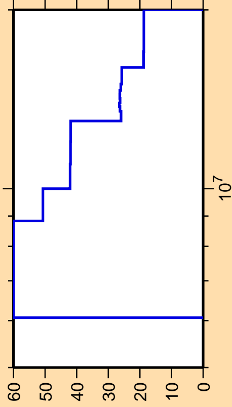
\Delta\sigma/\sigma vs. E for ^{244}\text{Es}(n,f)
