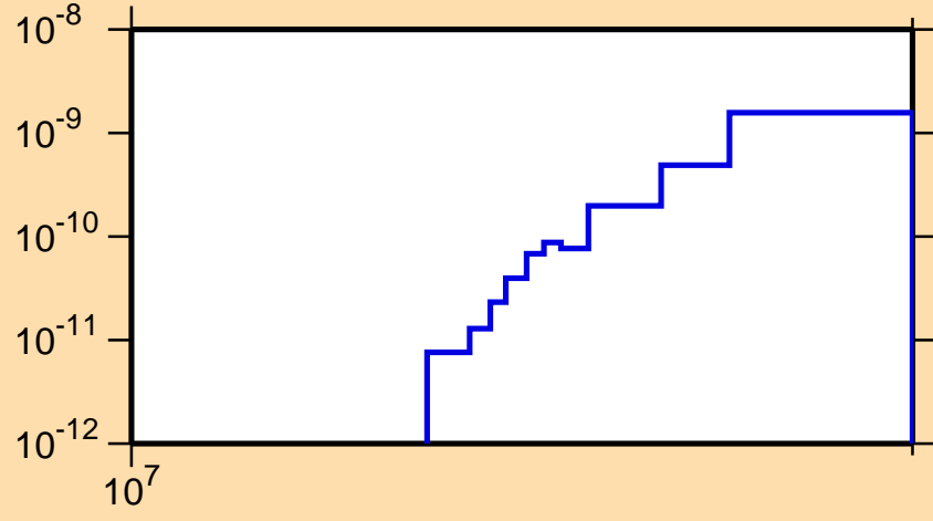
\sigma vs. E for ^{244}\text{Es}(\text{mt117})
