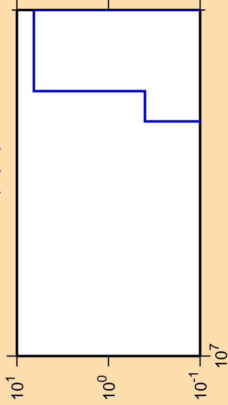
\Delta\sigma/\sigma vs. E for ^{244}\text{Es}(n,\text{pd})
