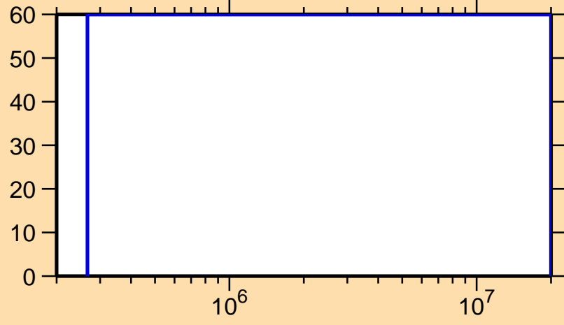
\Delta\sigma/\sigma vs. E for ^{244}\text{Es}(n,ncont.)
