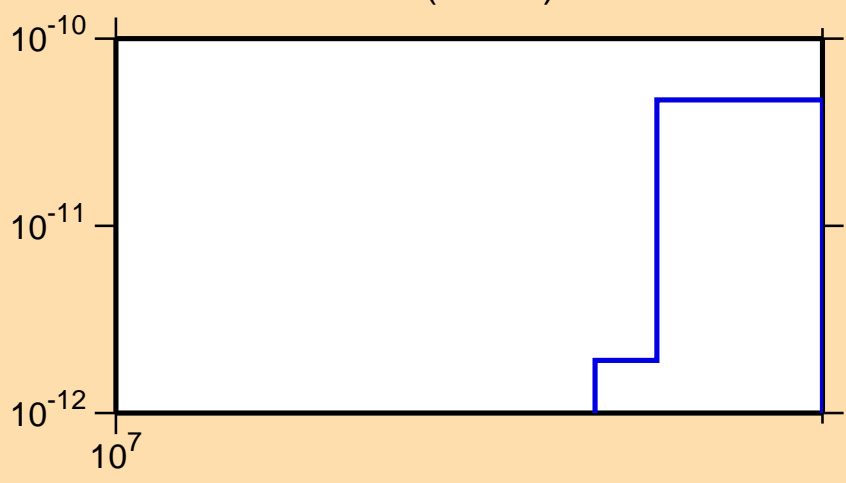
\sigma vs. E for ^{244}\text{Es} (mt 34)
