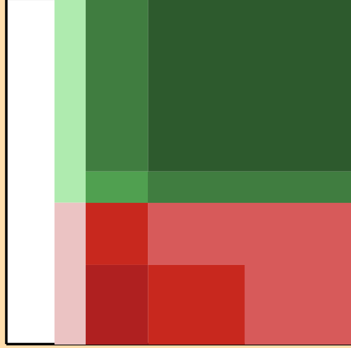
\Delta\sigma/\sigma vs. E for ^{244}\text{Es}(n,2n)
