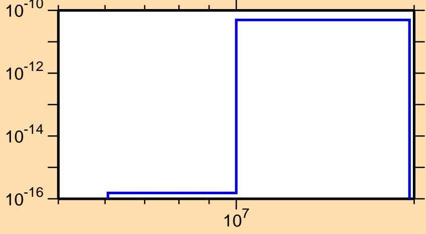
\sigma vs. E for ^{244}\text{Es}(\text{mt } 45)
