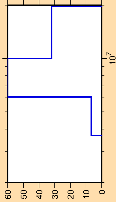
\Delta\sigma/\sigma vs. E for ^{244}\text{Es}(n,d)
