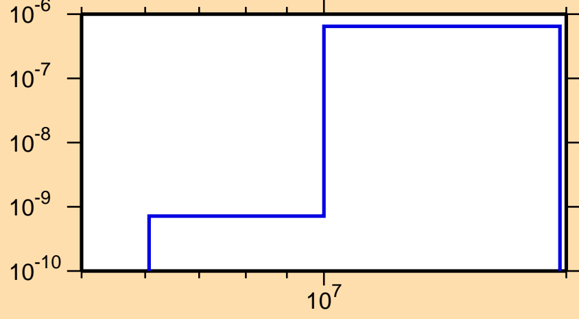
\sigma vs. E for ^{244}\text{Es}(n,2n\alpha)
