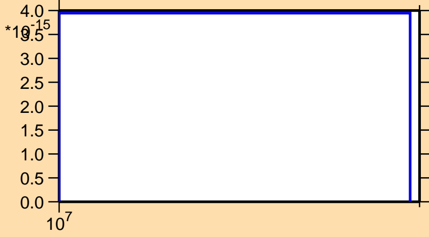
\sigma vs. E for ^{244}\text{Es}(n,\text{pt})
