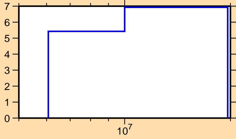
\Delta\sigma/\sigma vs. E for ^{244}\text{Es}(n,\text{tot.})
