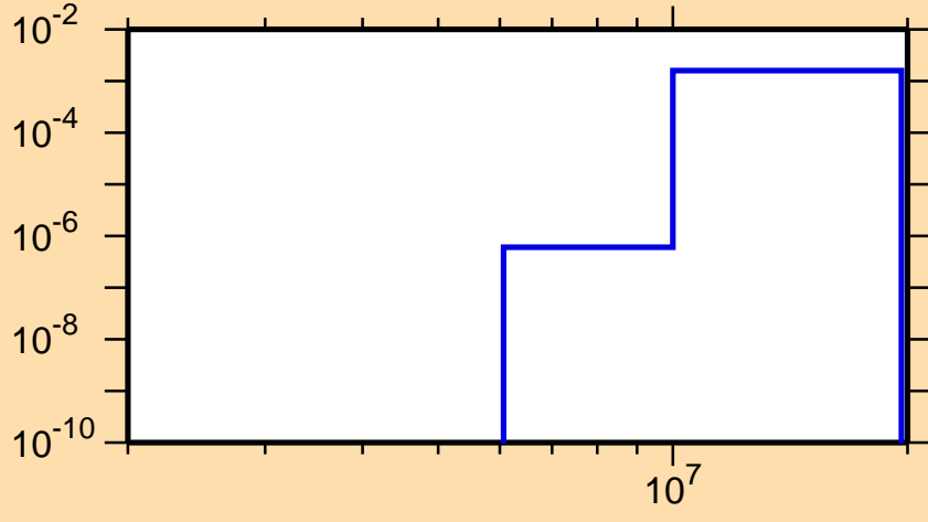
\sigma vs. E for ^{244}\text{Es}(n,d)
