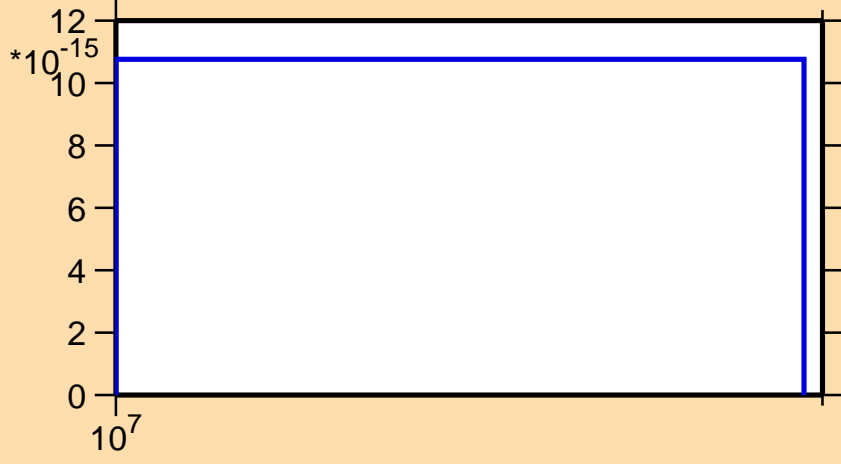
\sigma vs. E for ^{244}\text{Es}(n,\text{pd})
