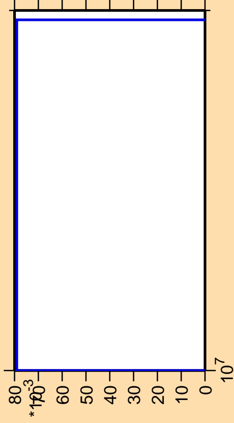
\Delta\sigma/\sigma vs. E for ^{244}\text{Es}(n,\text{pd})
