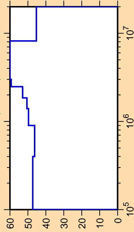
\Delta\sigma/\sigma vs. E for ^{244}\text{Es}(n,\text{inel.})
