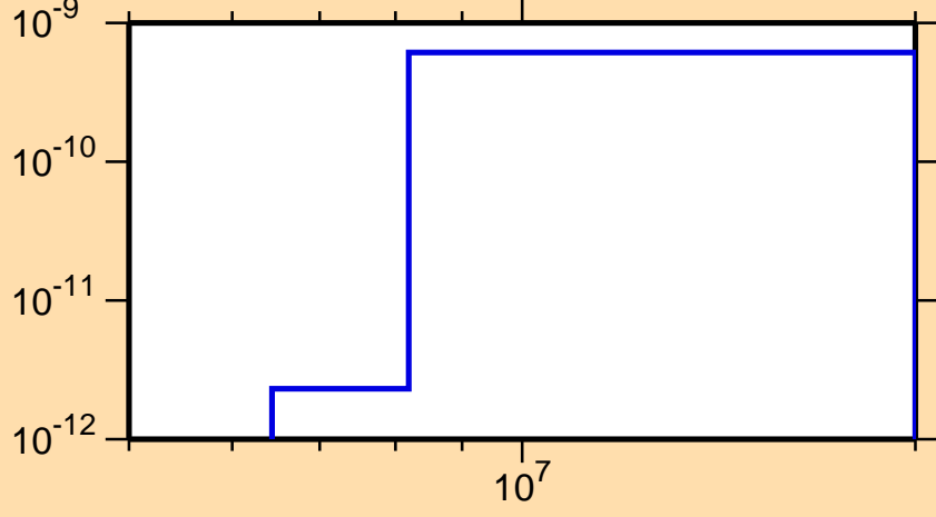
\sigma vs. E for ^{244}\text{Es}(n,p\alpha)
