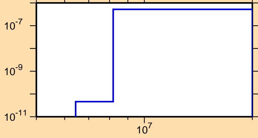
\sigma vs. E for ^{244}\text{Es}(n,2n\alpha)
