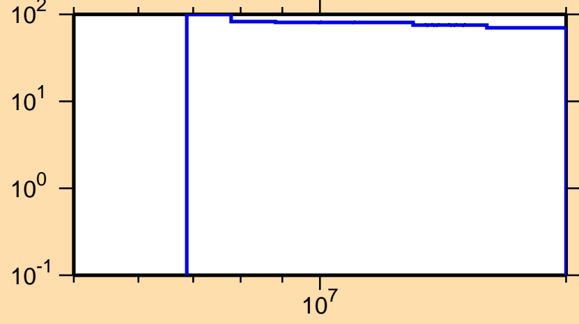
\Delta\sigma/\sigma vs. E for ^{245}\text{Es}(n,2n)
