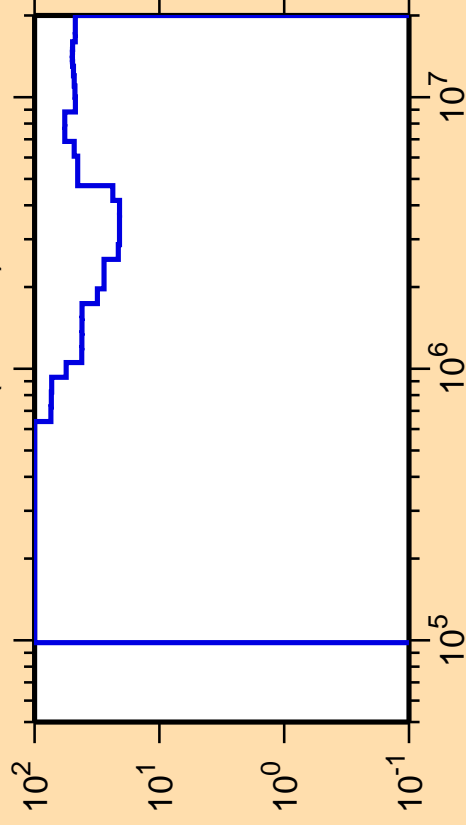
\Delta\sigma/\sigma vs. E for ^{245}\text{Es}(n,\text{inel.})
