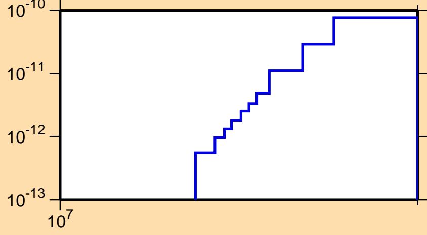
\sigma vs. E for ^{245}\text{Es}(\text{mt117})
