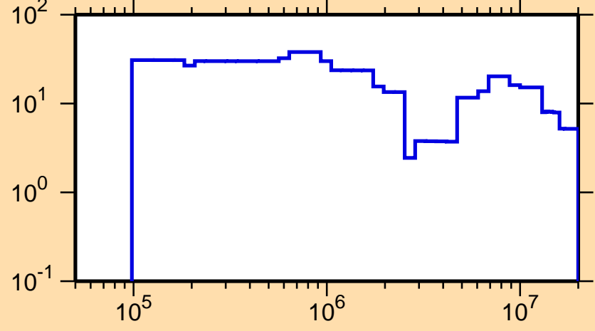
\Delta\sigma/\sigma vs. E for ^{245}\text{Es}(n,\text{tot.})
