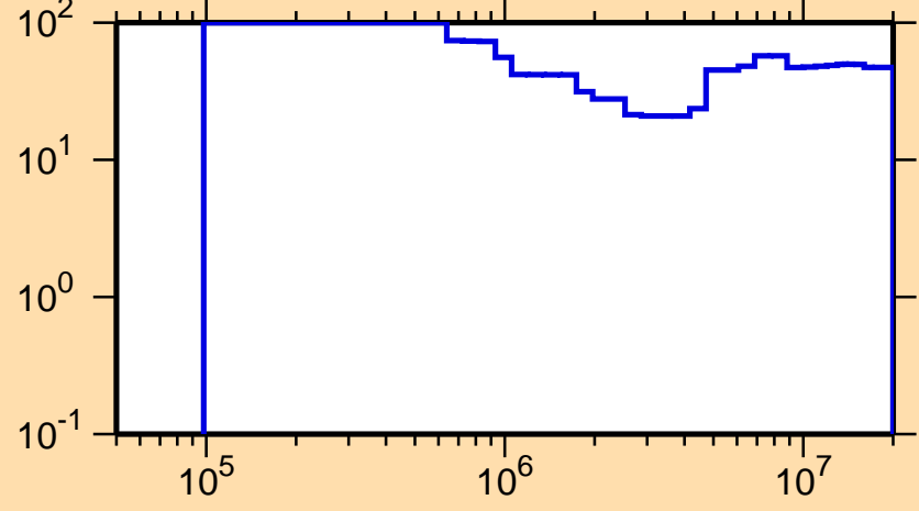
\Delta\sigma/\sigma vs. E for ^{245}\text{Es}(n,\text{inel.})
