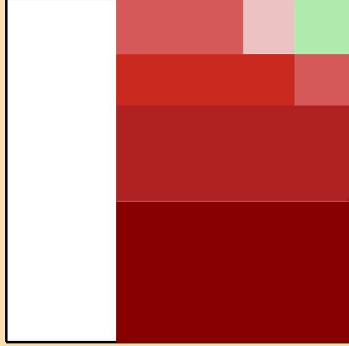
\Delta\sigma/\sigma vs. E for ^{245}\text{Es}(n,2n)
