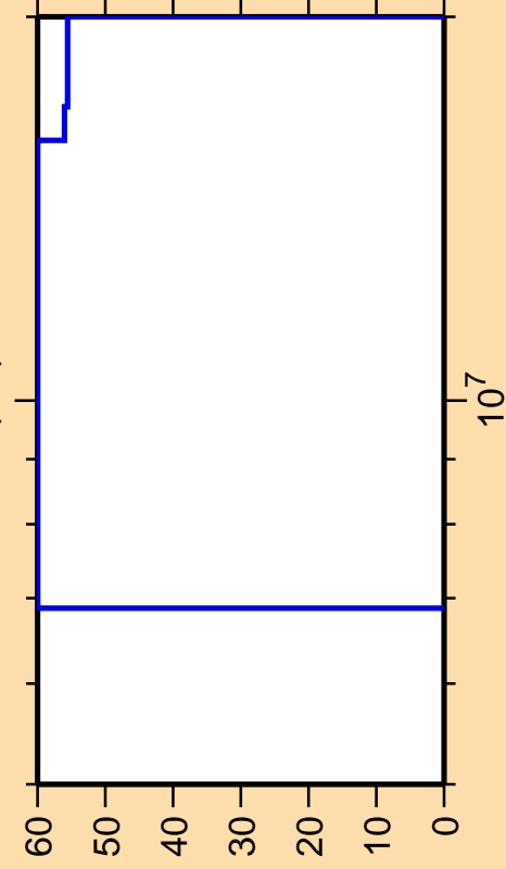
\Delta\sigma/\sigma vs. E for ^{245}\text{Es}(n,f)
