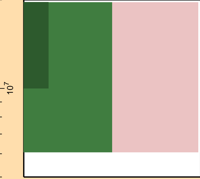
\Delta\sigma/\sigma vs. E for ^{245}\text{Es}(n,\text{inel.})
