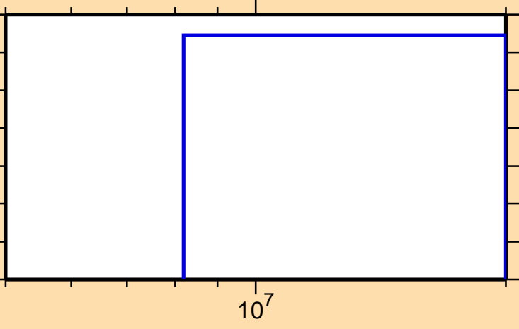
\sigma vs. E for ^{245}\text{Es}(n,nt)
