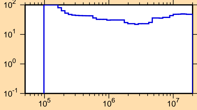
\Delta\sigma/\sigma vs. E for ^{246}\text{Es}(n,\text{inel.})
