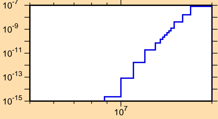
\sigma vs. E for ^{246}\text{Es}(n,\text{He3})
