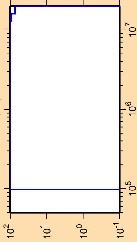
\Delta\sigma/\sigma vs. E for ^{246}\text{Es}(n,f)
