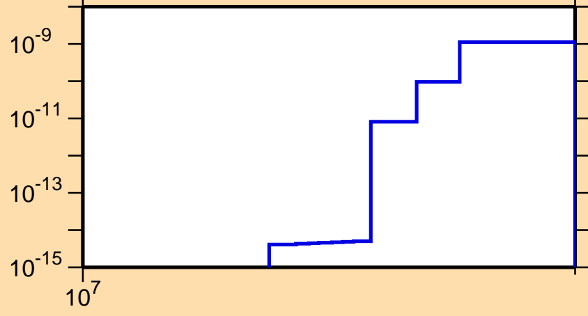
\sigma vs. E for ^{246}\text{Es}(n,3n\alpha)
