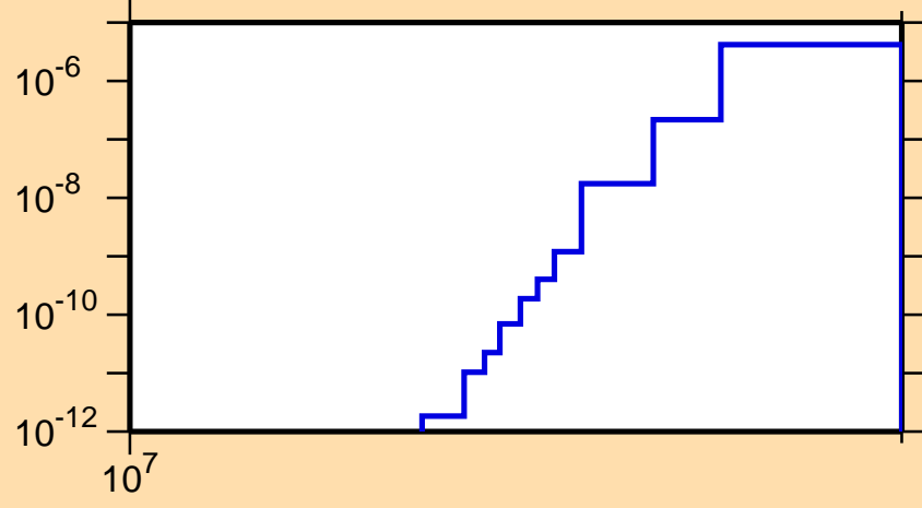
\sigma vs. E for ^{246}\text{Es}(n,nt)
