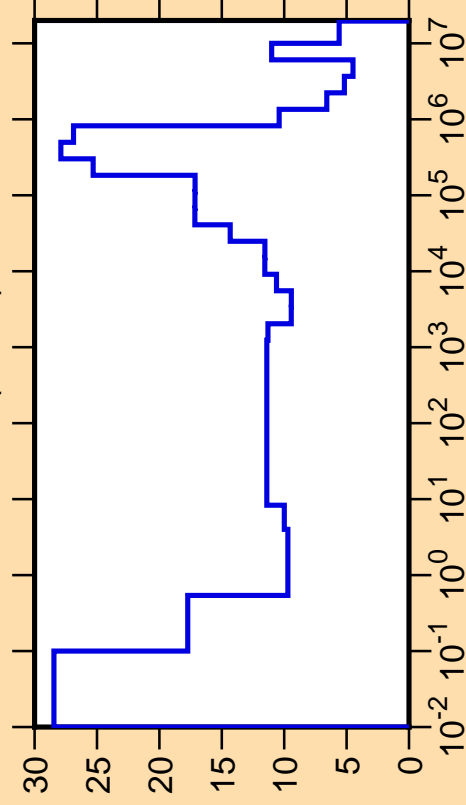
\Delta\sigma/\sigma vs. E for ^{246}\text{Es}(n,\text{tot.})
