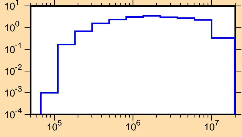
\sigma vs. E for ^{246}\text{Es}(n,\text{inel.})
