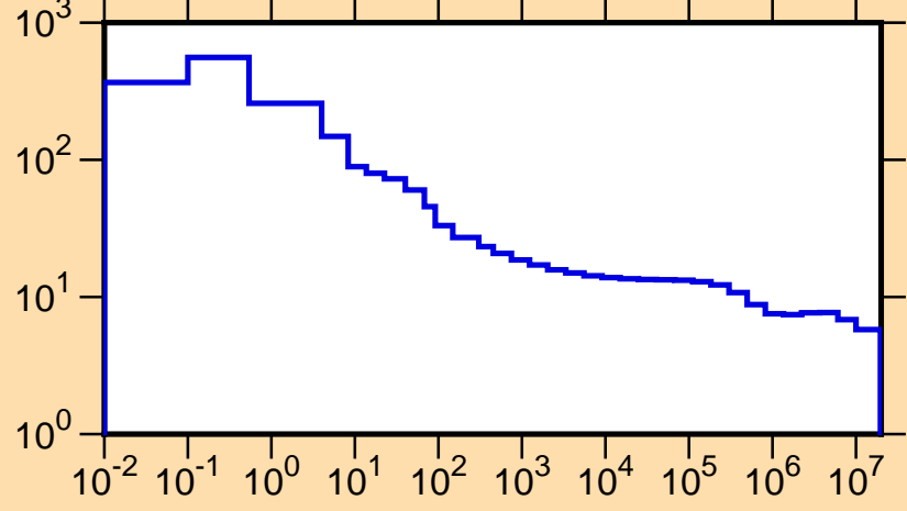
\sigma vs. E for ^{246}\text{Es}(n,\text{tot.})
