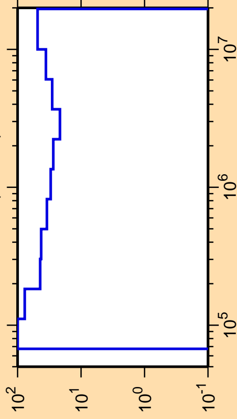
\Delta\sigma/\sigma vs. E for ^{246}\text{Es}(n,\text{inel.})
