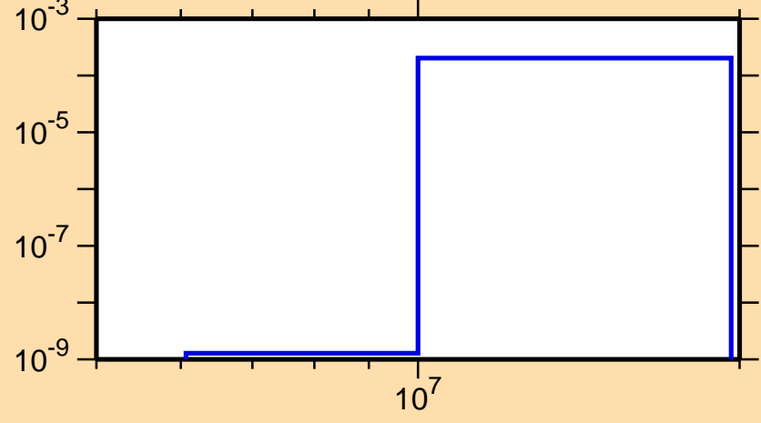
\sigma vs. E for ^{246}\text{Es}(n,t)
