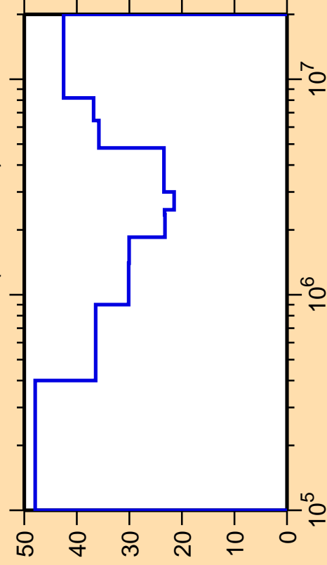
\Delta\sigma/\sigma vs. E for ^{246}\text{Es}(n,\text{ncont.})
