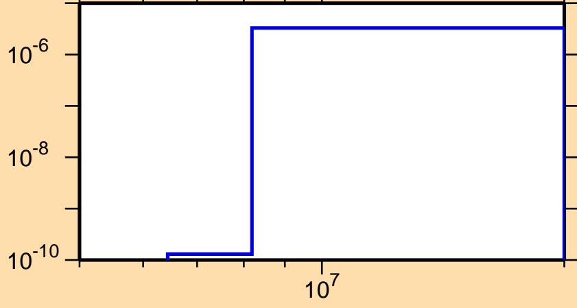
\sigma vs. E for ^{246}\text{Es}(n,2n\alpha)
