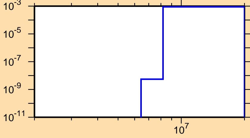
\sigma vs. E for ^{246}\text{Es}(n,d)
