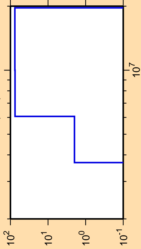
\Delta\sigma/\sigma vs. E for ^{247}\text{Es}(n,d)
