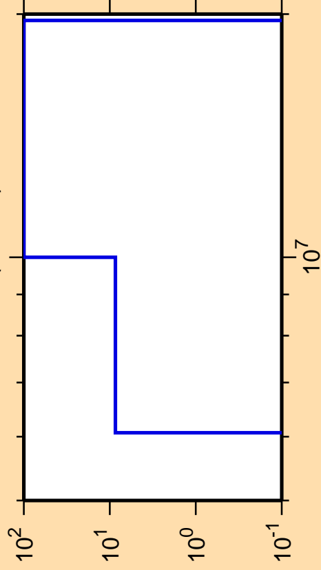
\Delta\sigma/\sigma vs. E for ^{247}\text{Es}(n,2n\alpha)
