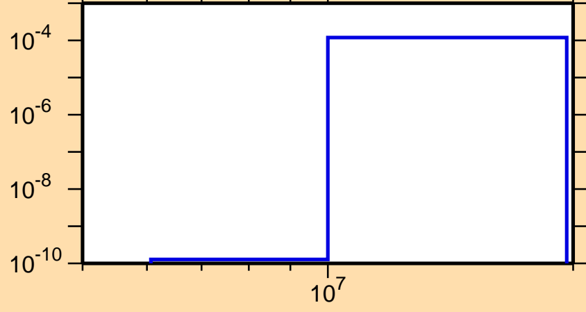
\sigma vs. E for ^{247}\text{Es}(n,t)
