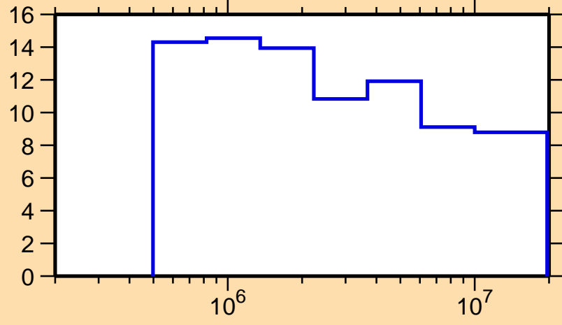
\Delta\sigma/\sigma vs. E for ^{247}\text{Es}(n, n_{\text{nonel.}})
