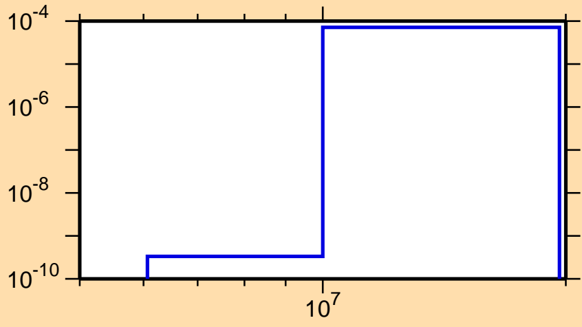
\sigma vs. E for ^{247}\text{Es}(\text{mt } 45)
