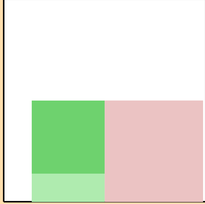
\Delta\sigma/\sigma vs. E for ^{247}\text{Es}(n,2n)
