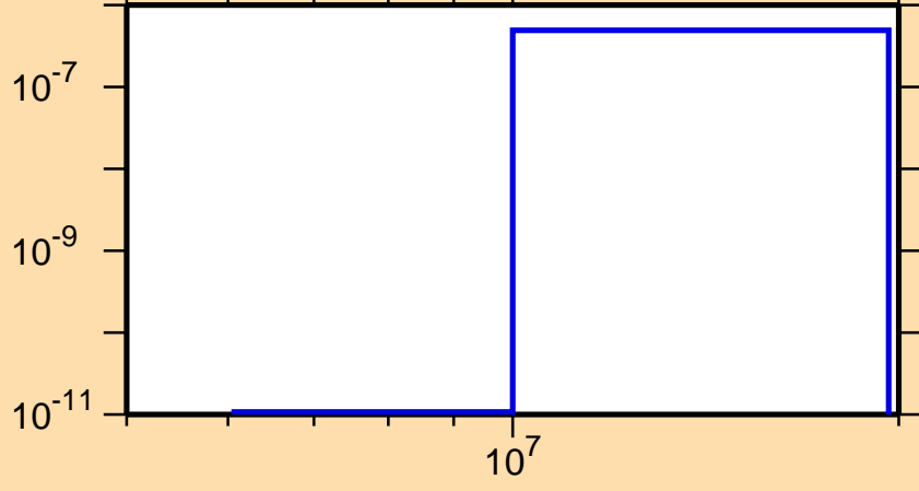
\sigma vs. E for ^{247}\text{Es}(n,2n\alpha)
