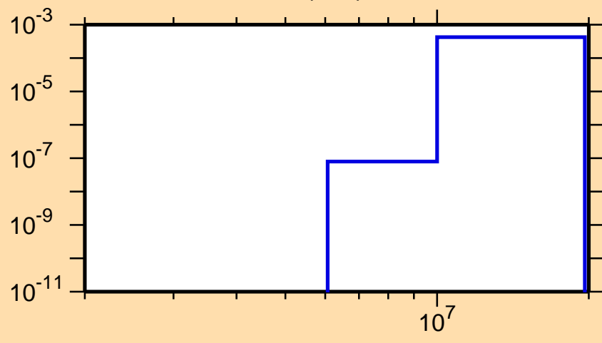
\sigma vs. E for ^{247}\text{Es}(n,d)
