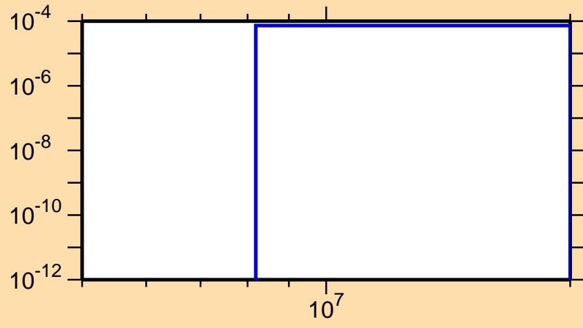
\sigma vs. E for ^{247}\text{Es}(\text{mt117})
