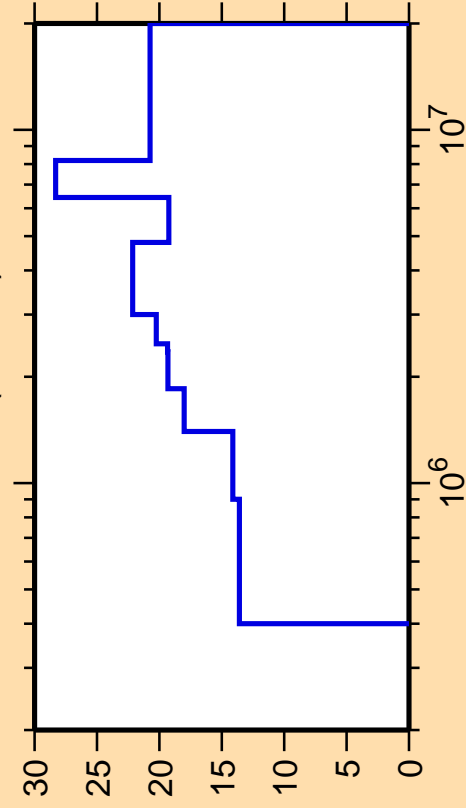
\Delta\sigma/\sigma vs. E for ^{247}\text{Es}(n,\text{inel.})
