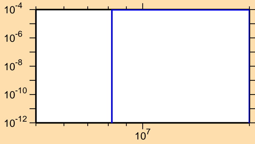
\sigma vs. E for ^{247}\text{Es}(n,t)
