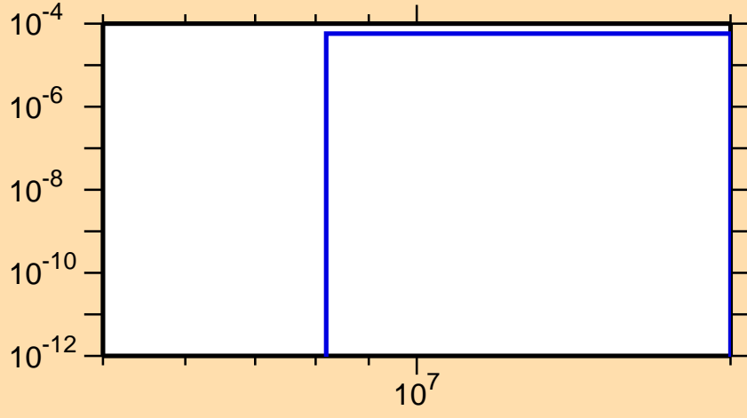
\sigma vs. E for ^{247}\text{Es} (mt 45)
