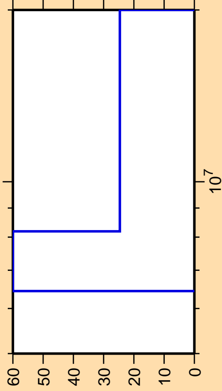
\Delta\sigma/\sigma vs. E for ^{247}\text{Es}(n,p)
