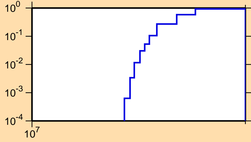
\sigma vs. E for ^{249}\text{Es}(n,3n)
