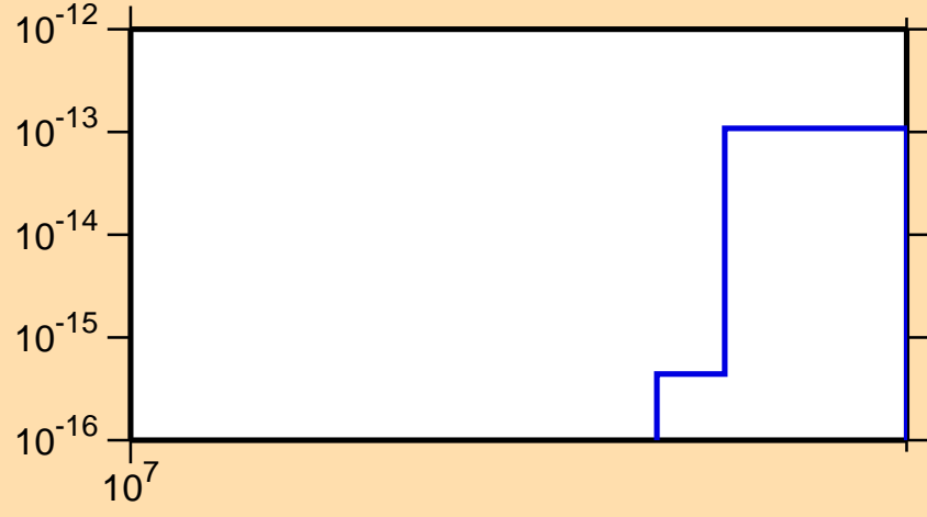
\sigma vs. E for ^{249}\text{Es} (mt 34)
