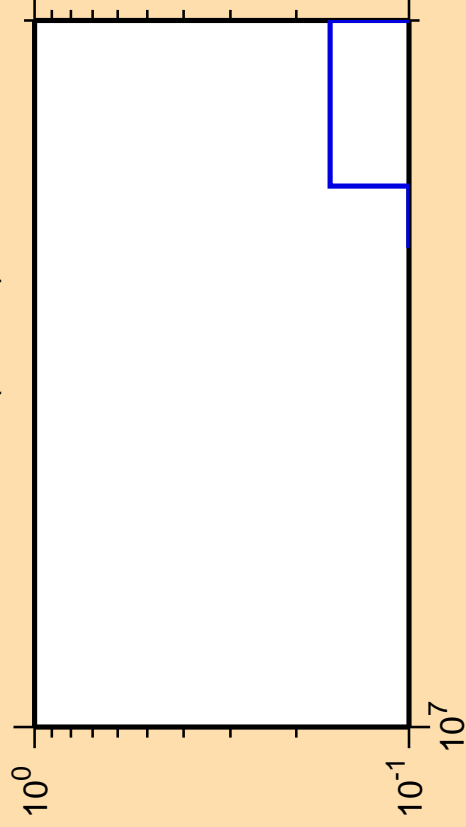
\Delta\sigma/\sigma vs. E for ^{249}\text{Es} (mt 42)
