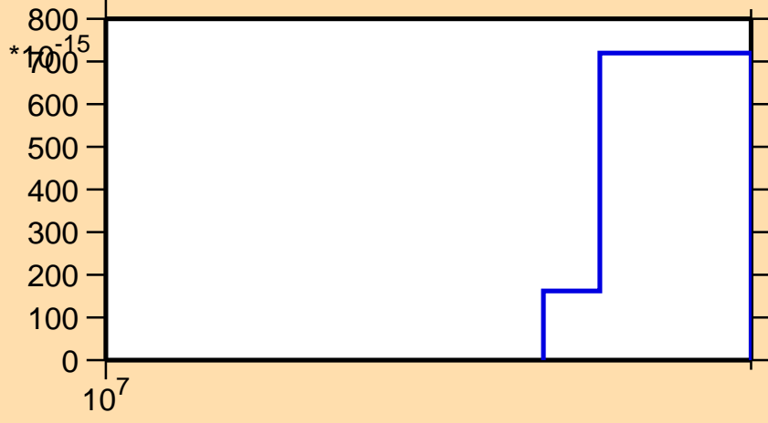
\sigma vs. E for ^{249}\text{Es} (mt 45)
