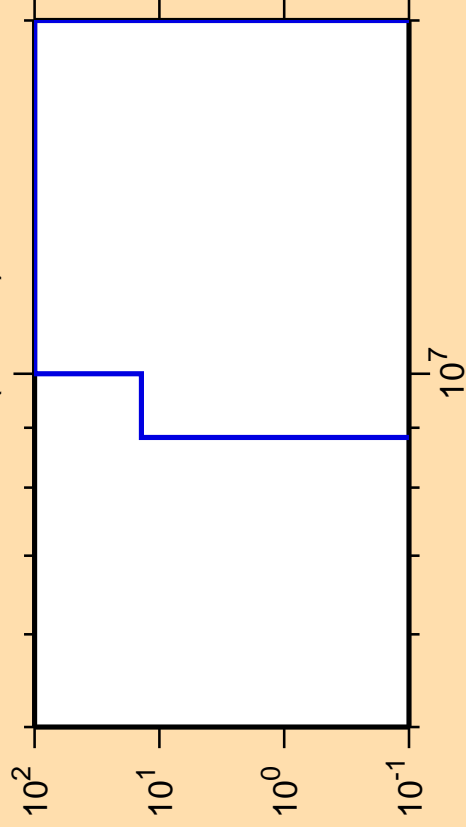
\Delta\sigma/\sigma vs. E for ^{249}\text{Es}(n,2n\alpha)
