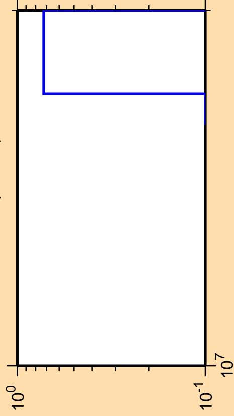
\Delta\sigma/\sigma vs. E for ^{249}\text{Es} (mt 34)
