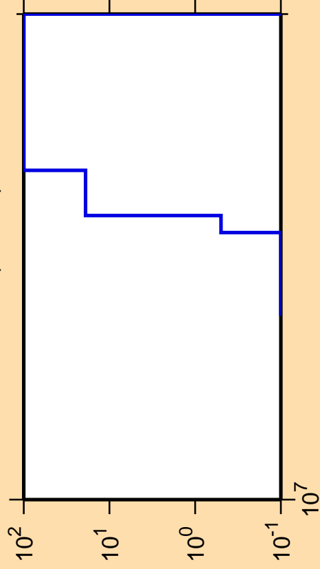
\Delta\sigma/\sigma vs. E for ^{249}\text{Es}(n,3n\alpha)
