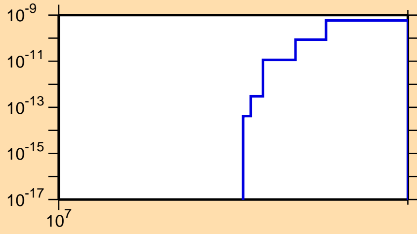
\sigma vs. E for ^{249}\text{Es}(n,3n\alpha)
