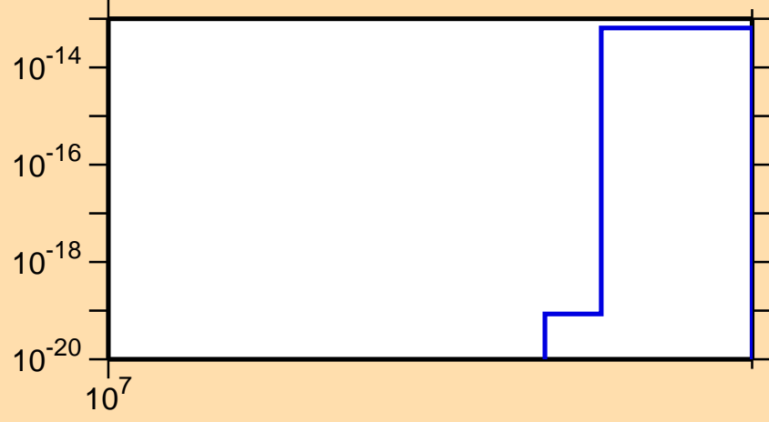
\sigma vs. E for ^{249}\text{Es} (mt 42)
