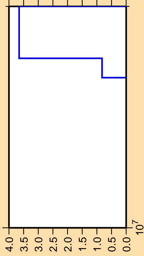
\Delta\sigma/\sigma vs. E for ^{249}\text{Es} (mt 45)
