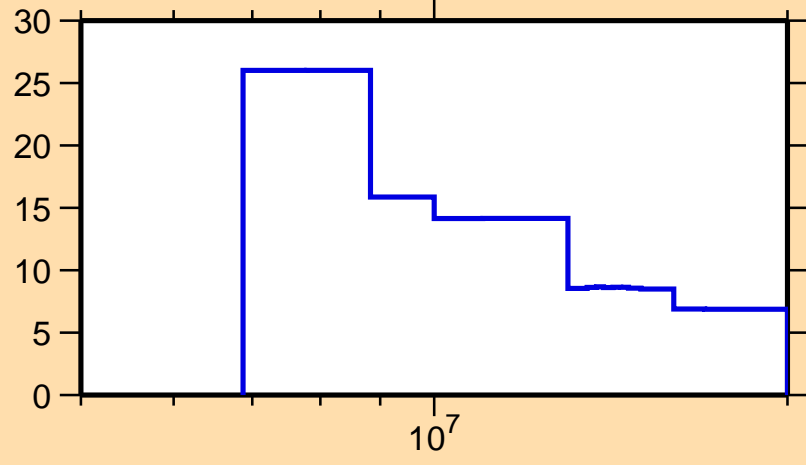
\Delta\sigma/\sigma vs. E for ^{249}\text{Es}(n,\text{el.})
