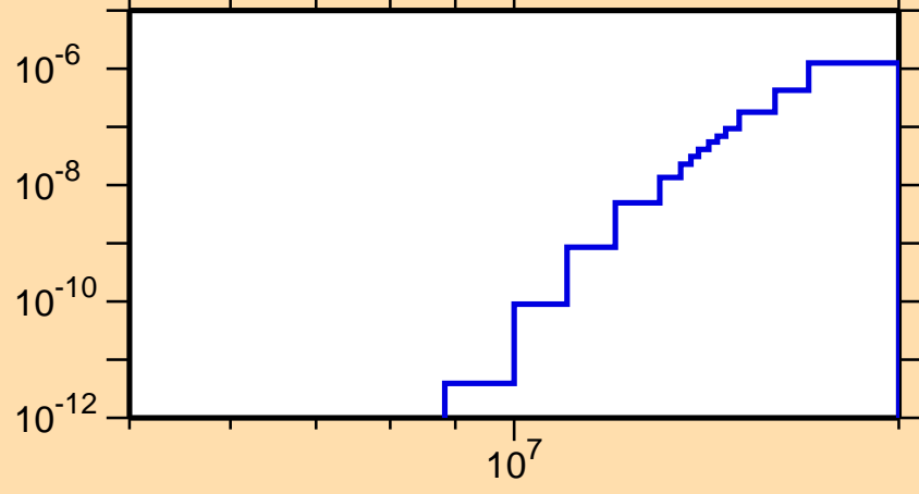
\sigma vs. E for ^{249}\text{Es}(n,2n\alpha)
