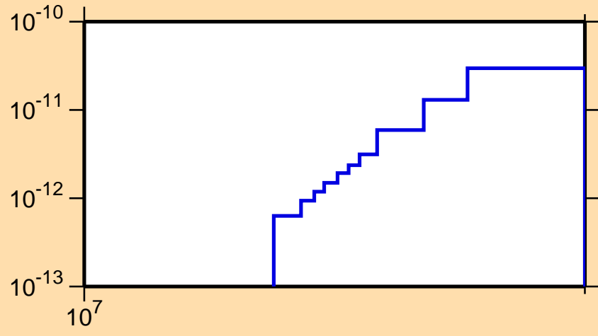
\sigma vs. E for ^{249}\text{Es}(n,p\alpha)
