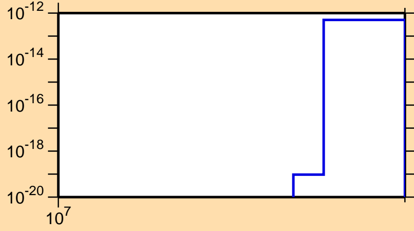
\sigma vs. E for ^{249}\text{Es} (mt 11)
