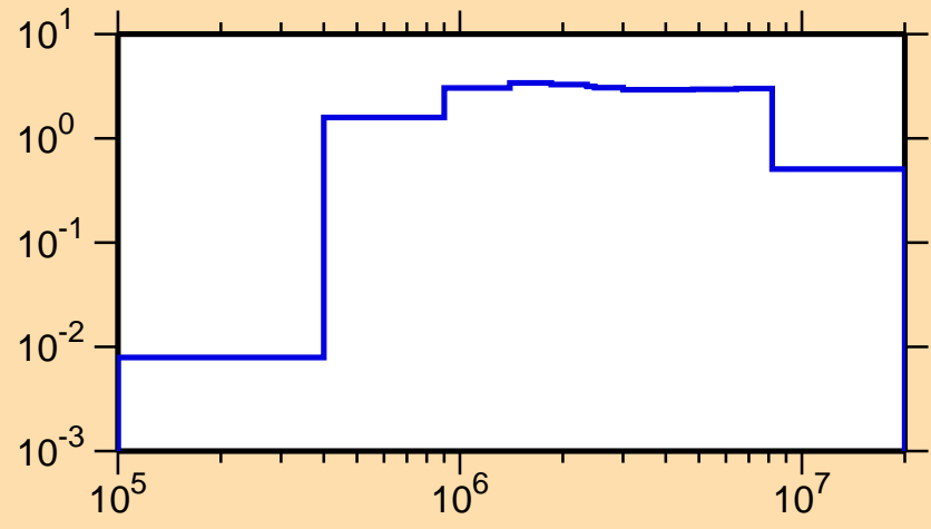
\sigma vs. E for ^{249}\text{Es}(n,\text{inel.})
