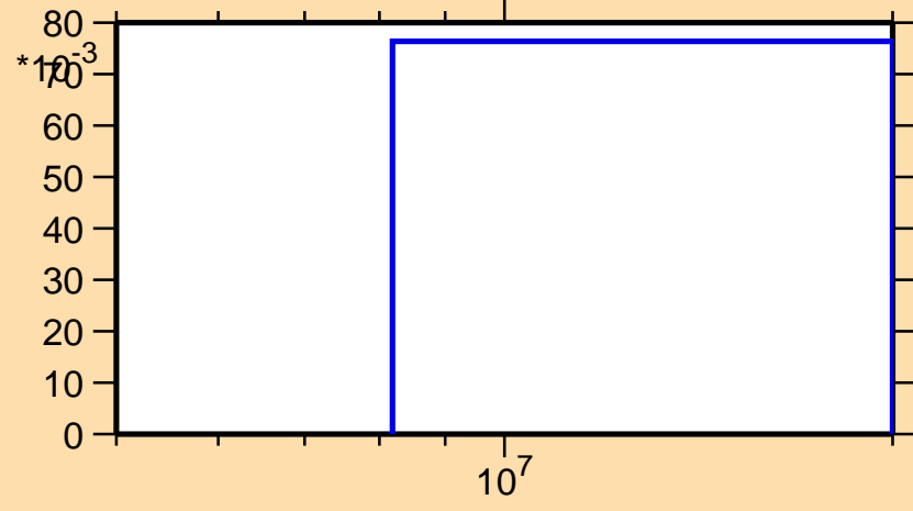
\sigma vs. E for ^{249}\text{Es}(n,3n)
