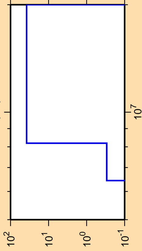
\Delta\sigma/\sigma vs. E for ^{249}\text{Es}(n,t)
