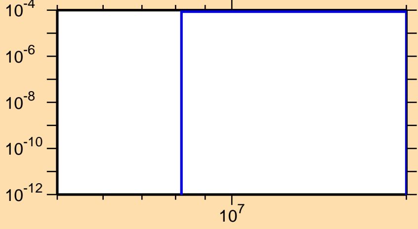
\sigma vs. E for ^{249}\text{Es}(n,t)
