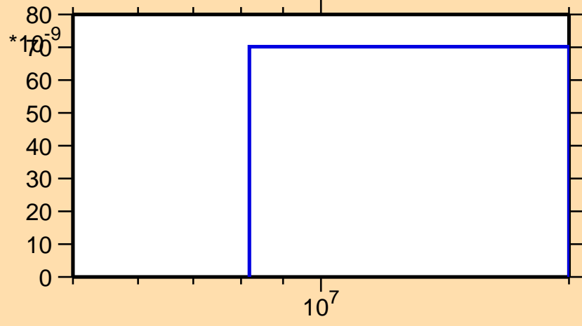
\sigma vs. E for ^{249}\text{Es}(n,2np)
