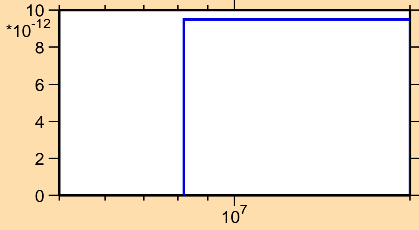
\sigma vs. E for ^{249}\text{Es}(n,3n\alpha)
