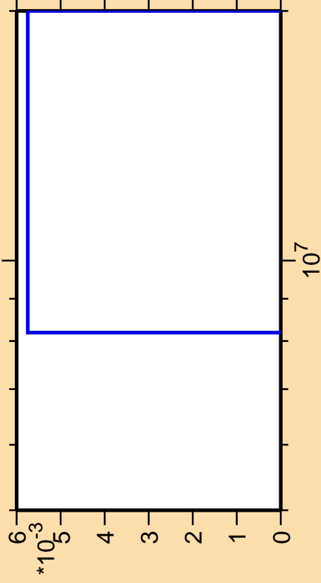
\Delta\sigma/\sigma vs. E for ^{249}\text{Es} (mt 11)
