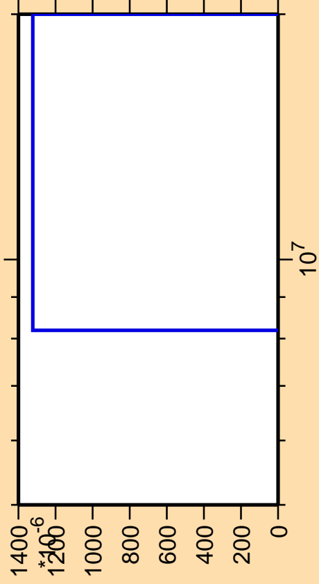
\Delta\sigma/\sigma vs. E for ^{249}\text{Es} (mt 42)
