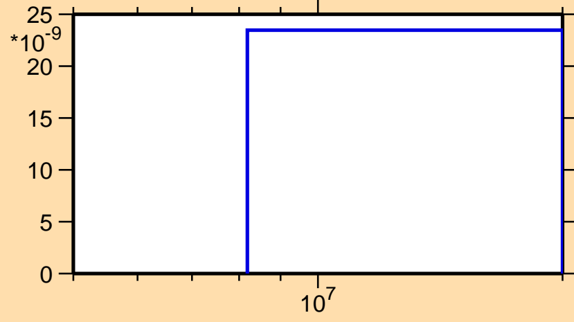
\sigma vs. E for ^{249}\text{Es}(n,nt)
