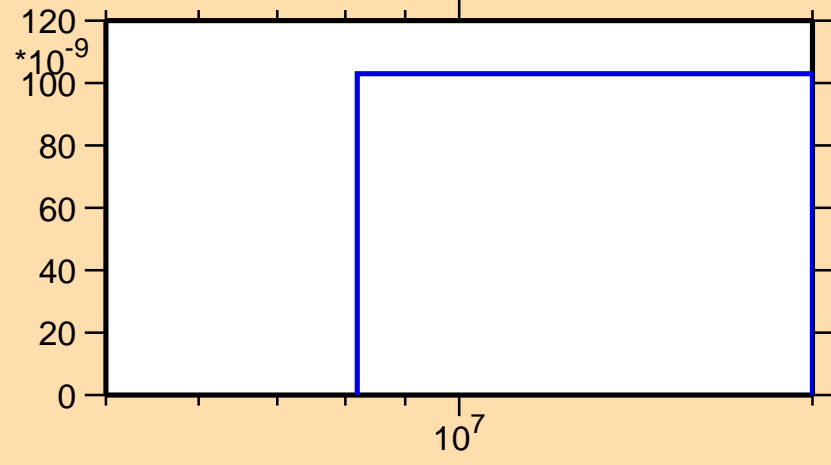
\sigma vs. E for ^{249}\text{Es}(n,nd)
