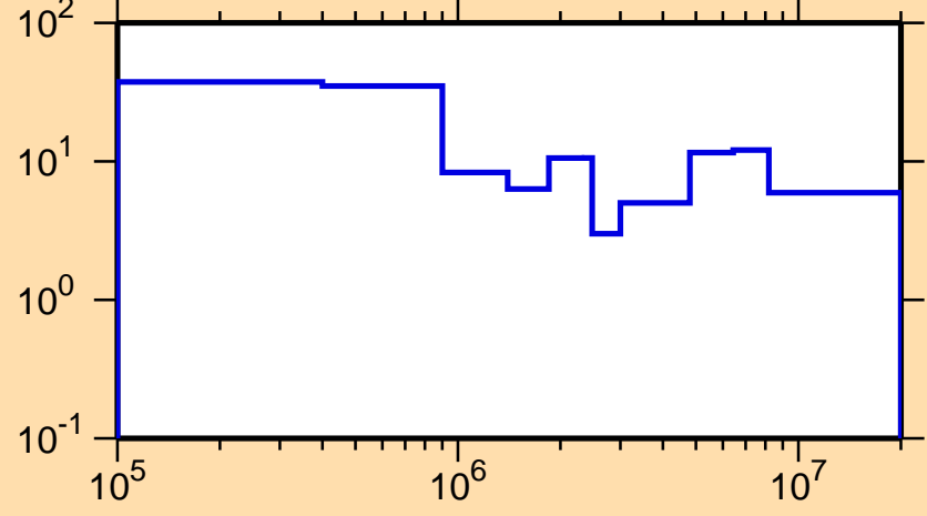
\Delta\sigma/\sigma vs. E for ^{249}\text{Es}(n,\text{tot.})
