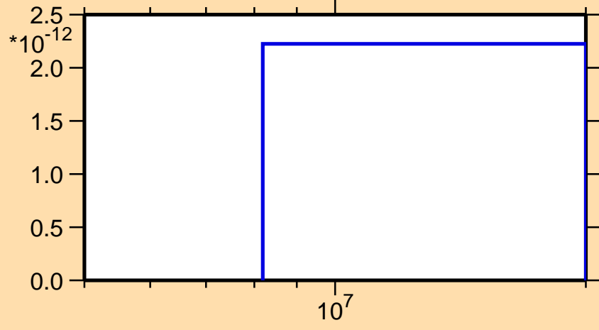
\sigma vs. E for ^{249}\text{Es}(n,p\alpha)
