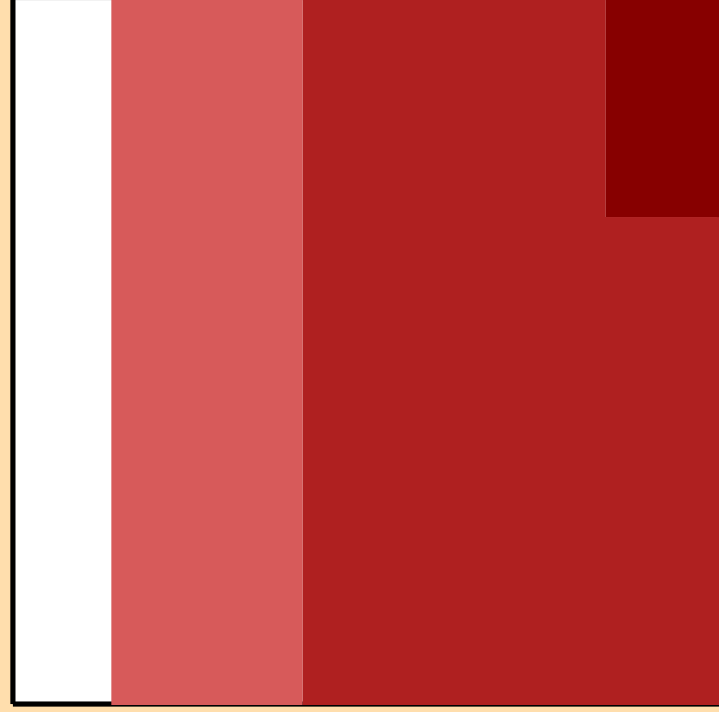
\Delta\sigma/\sigma vs. E for ^{250}\text{Es}(n,2n)
