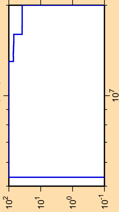
\Delta\sigma/\sigma vs. E for ^{250}\text{Es}(n,\alpha)
