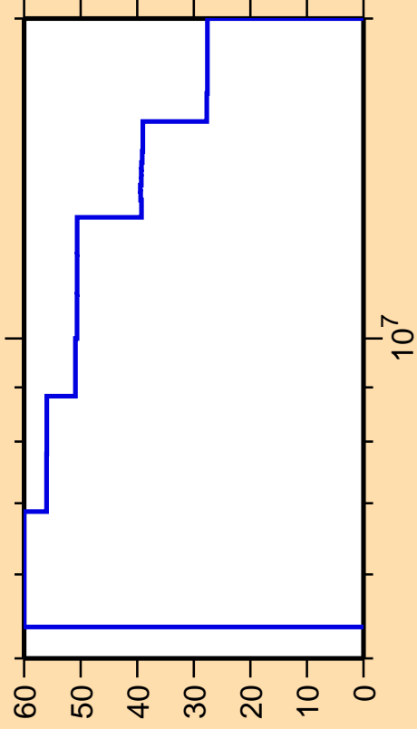
\Delta\sigma/\sigma vs. E for ^{250}\text{Es}(n,p)
