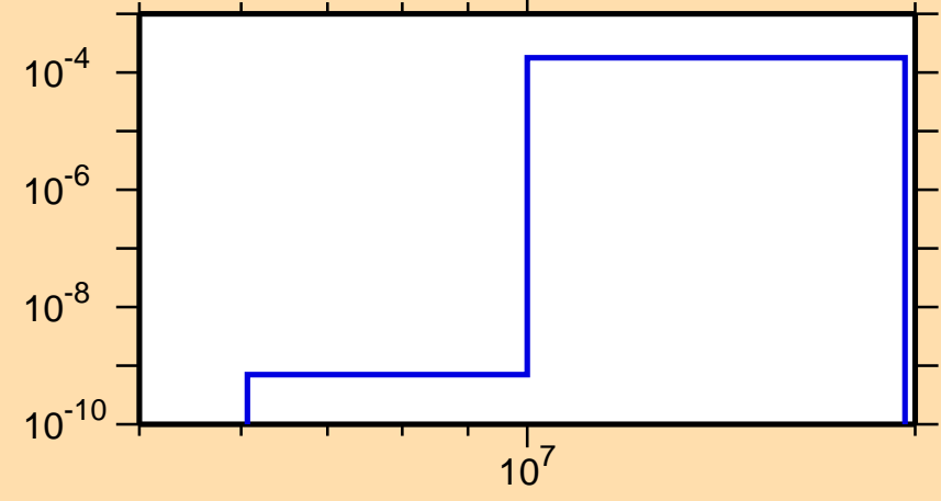
\sigma vs. E for ^{250}\text{Es}(n,t)
