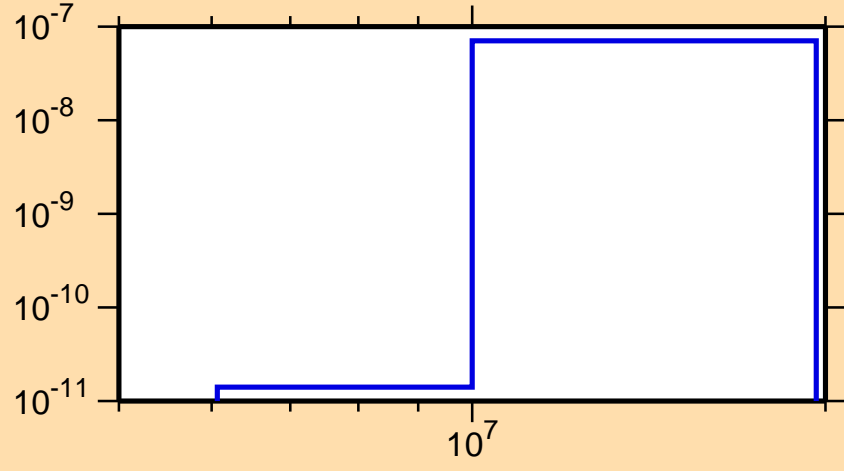
\sigma vs. E for ^{250}\text{Es}(n,2n\alpha)
