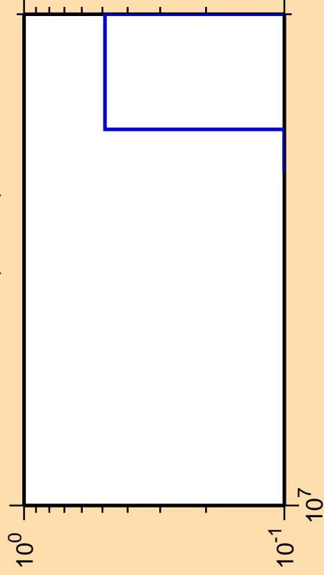
\Delta\sigma/\sigma vs. E for ^{251}\text{Es} (mt 42)
