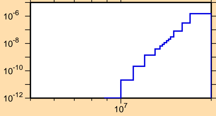
\sigma vs. E for ^{251}\text{Es}(n,2n\alpha)
