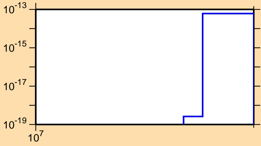
\sigma vs. E for ^{251}\text{Es} (mt 42)
