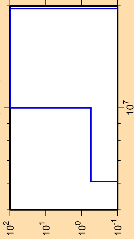
\Delta\sigma/\sigma vs. E for ^{251}\text{Es}(n,2n\alpha)
