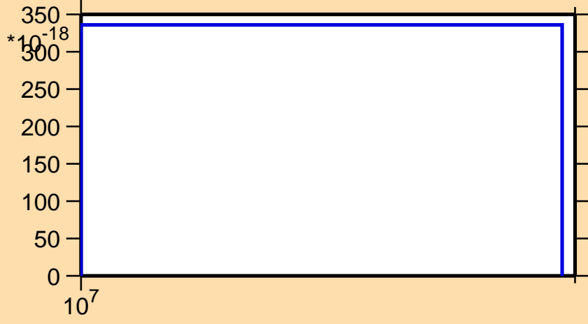
\sigma vs. E for ^{251}\text{Es} (mt 42)
