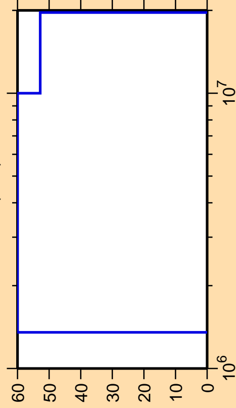
\Delta\sigma/\sigma vs. E for ^{251}\text{Es}(n,\alpha)
