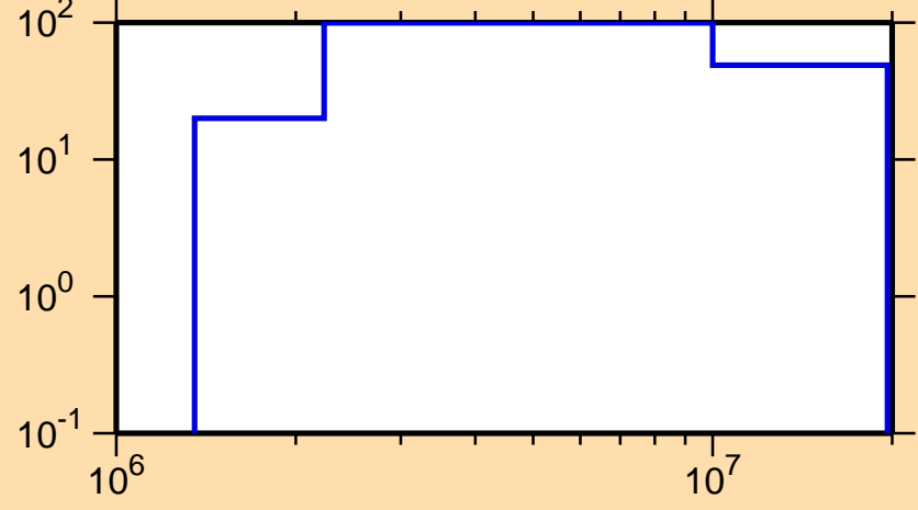
\Delta\sigma/\sigma vs. E for ^{251}\text{Es}(n,p)
