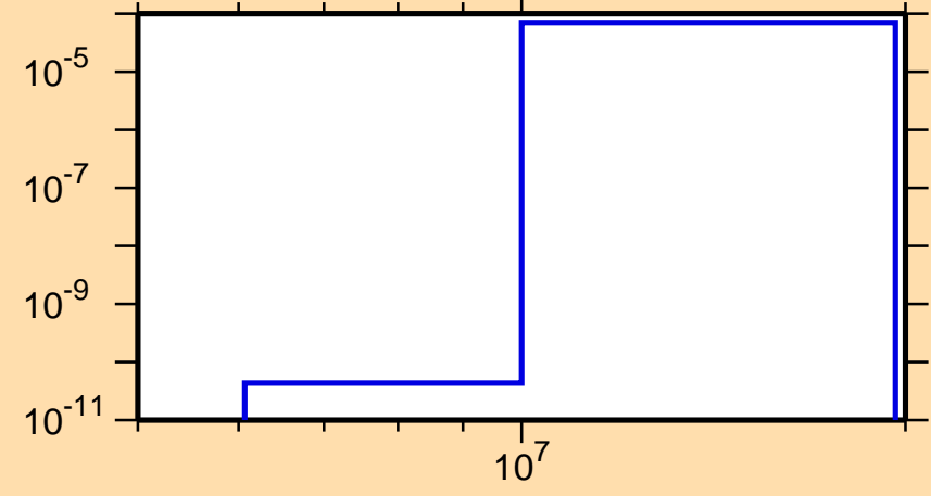
\sigma vs. E for ^{251}\text{Es}(n,t)
