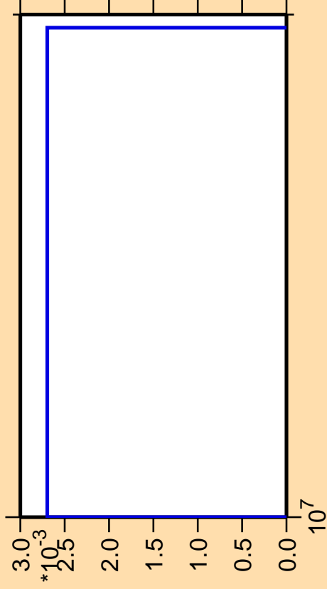
\Delta\sigma/\sigma vs. E for ^{251}\text{Es} (mt 42)
