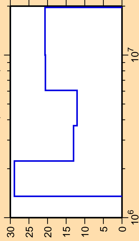
\Delta\sigma/\sigma vs. E for ^{251}\text{Es}(n,\text{ncont.})
