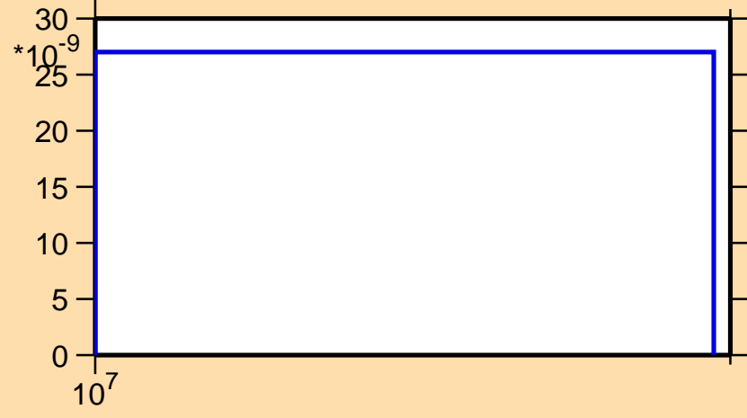
\sigma vs. E for ^{251}\text{Es}(n,2np)
