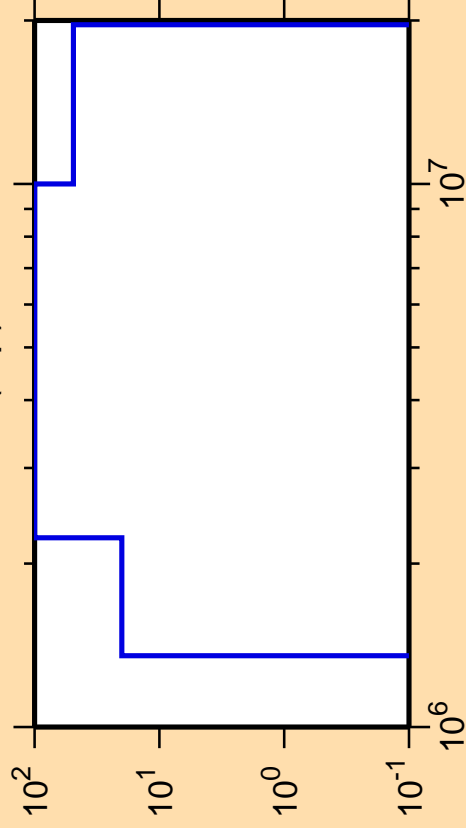
\Delta\sigma/\sigma vs. E for ^{251}\text{Es}(n,p)
