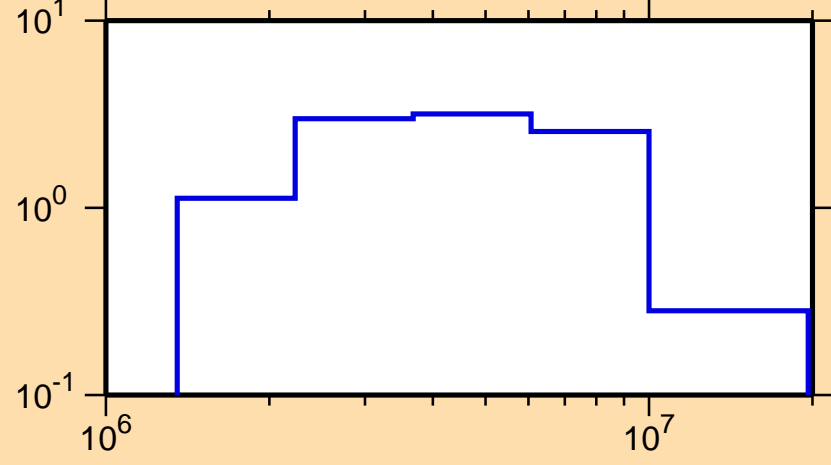
\sigma vs. E for ^{251}\text{Es}(n,n\text{cont.})
