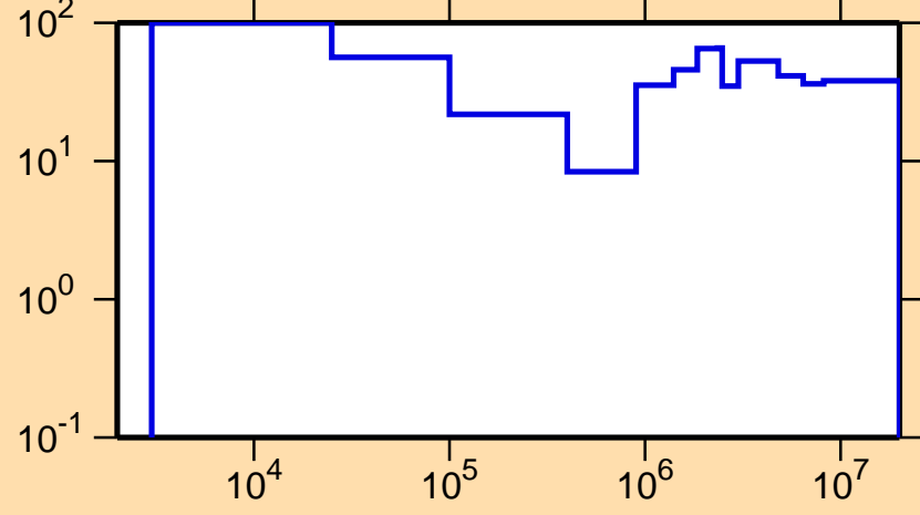
\Delta\sigma/\sigma vs. E for ^{251}\text{Es}(n,n_1)
