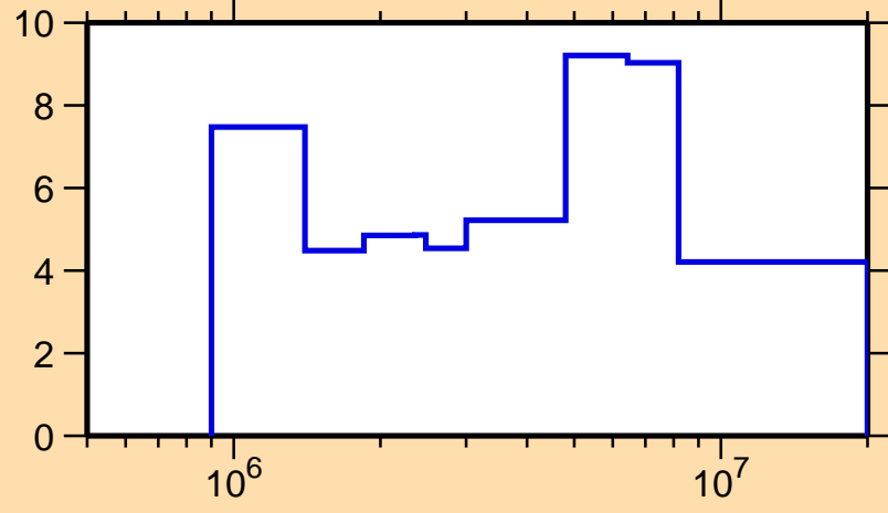
\Delta\sigma/\sigma vs. E for ^{251}\text{Es}(n, tot.)
