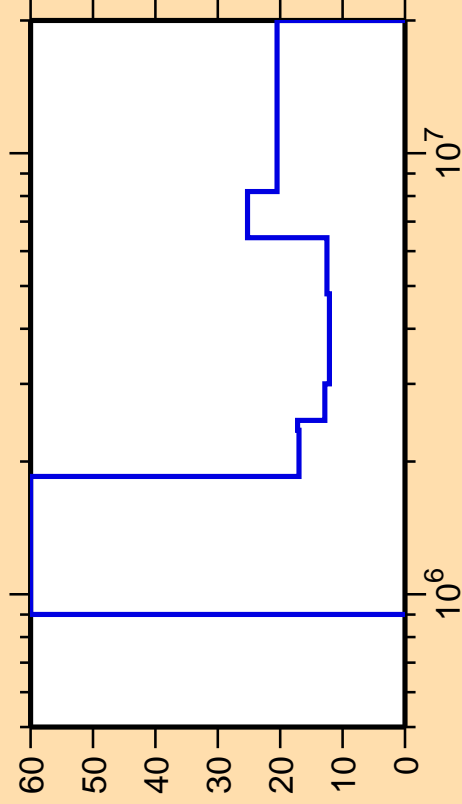
\Delta\sigma/\sigma vs. E for ^{251}\text{Es}(n, ncont.)
