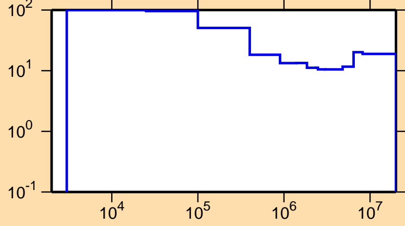
\Delta\sigma/\sigma vs. E for ^{251}\text{Es}(n,\text{inel.})
