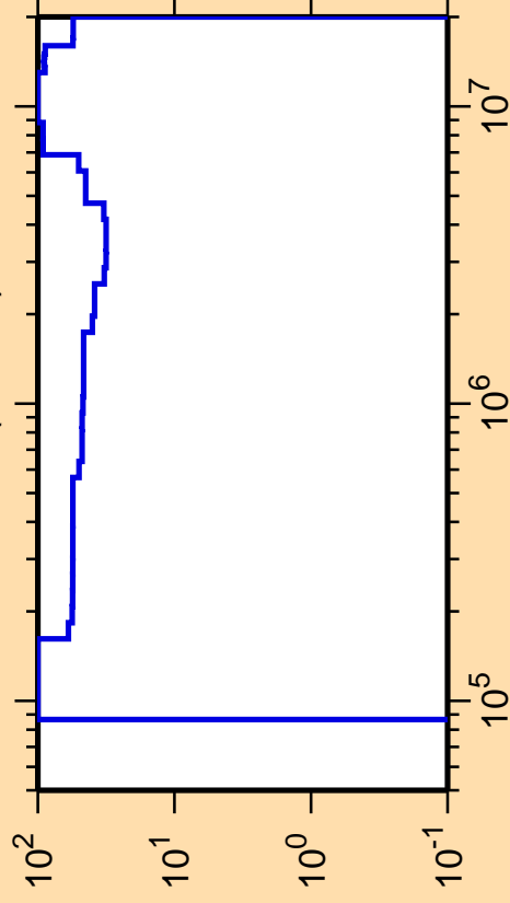
\Delta\sigma/\sigma vs. E for ^{252}\text{Es}(n,\text{inel.})
