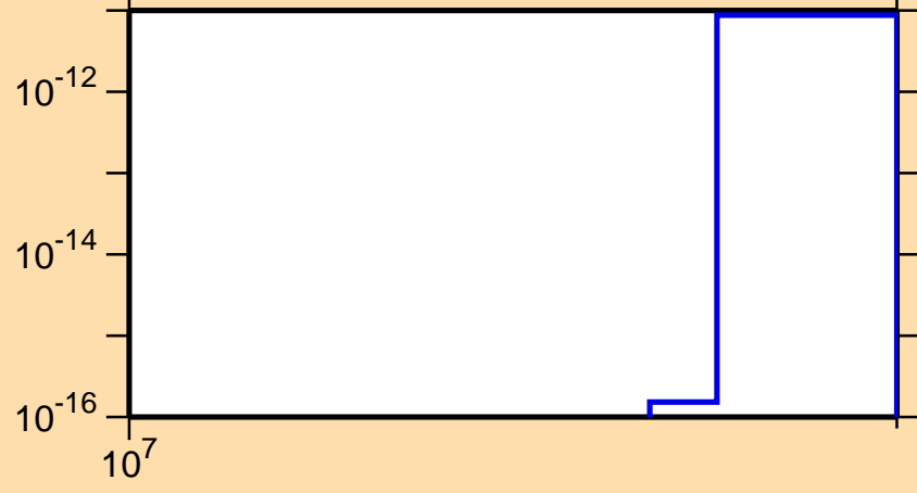
\sigma vs. E for ^{252}\text{Es} (mt 11)
