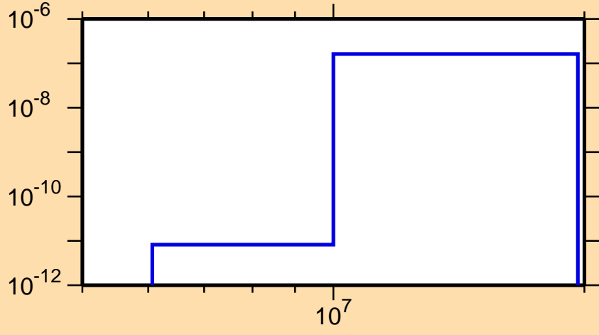
\sigma vs. E for ^{252}\text{Es}(n,2n\alpha)
