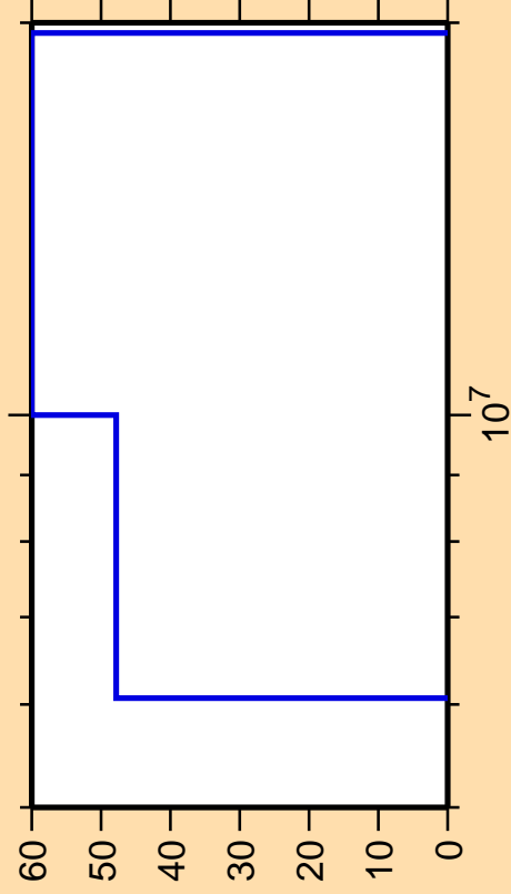
\Delta\sigma/\sigma vs. E for ^{252}\text{Es}(n,2n\alpha)
