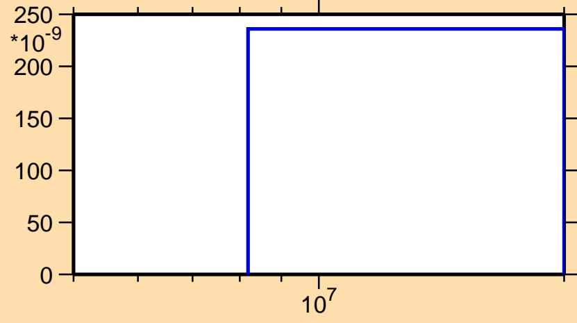
\sigma vs. E for ^{252}\text{Es}(n,nt)
