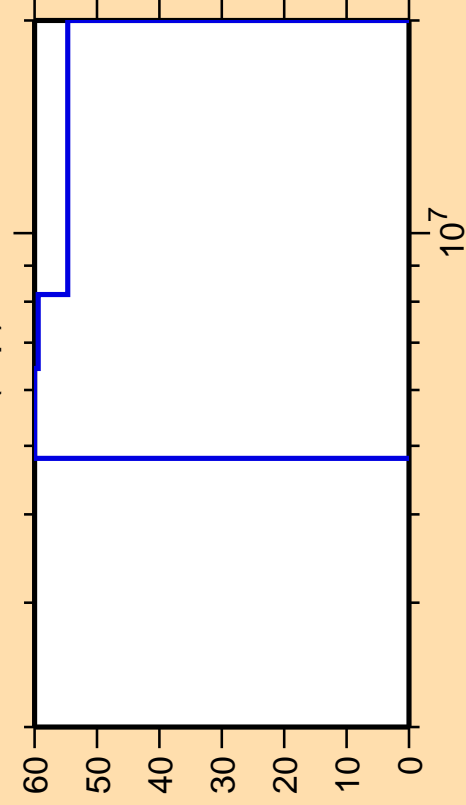
\Delta\sigma/\sigma vs. E for ^{252}\text{Es}(n,p)
