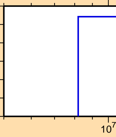
\sigma vs. E for ^{252}\text{Es}(n,3n\alpha)
