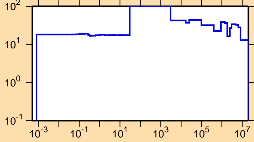
\Delta\sigma/\sigma vs. E for ^{252}\text{Es}(n,\text{el.})
