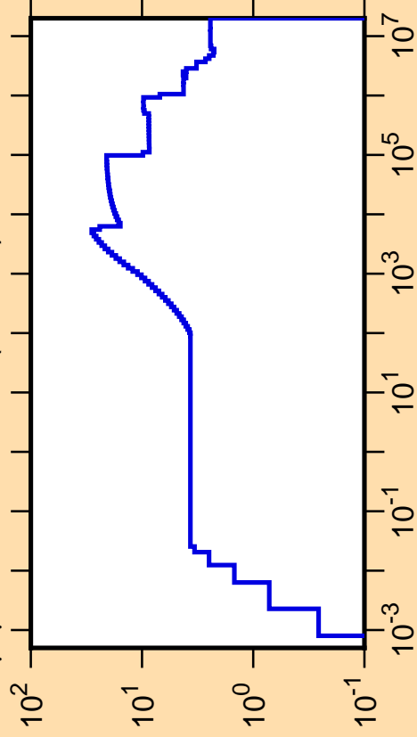
\Delta\mu/\mu vs. E for ^{253}\text{Es}(\text{mt251})
