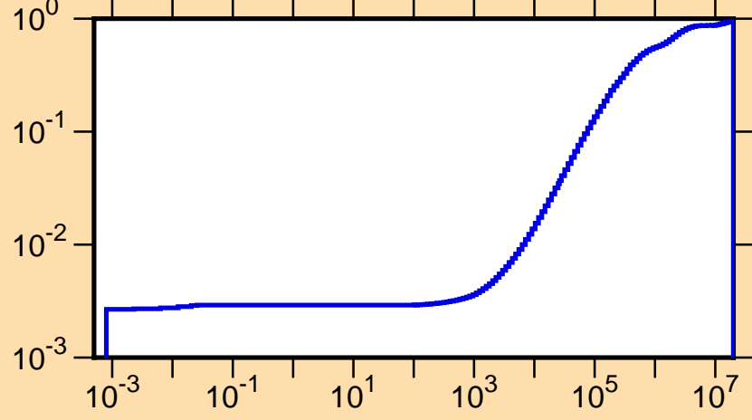
\mu vs. E for ^{253}\text{Es}(\text{mt251})
