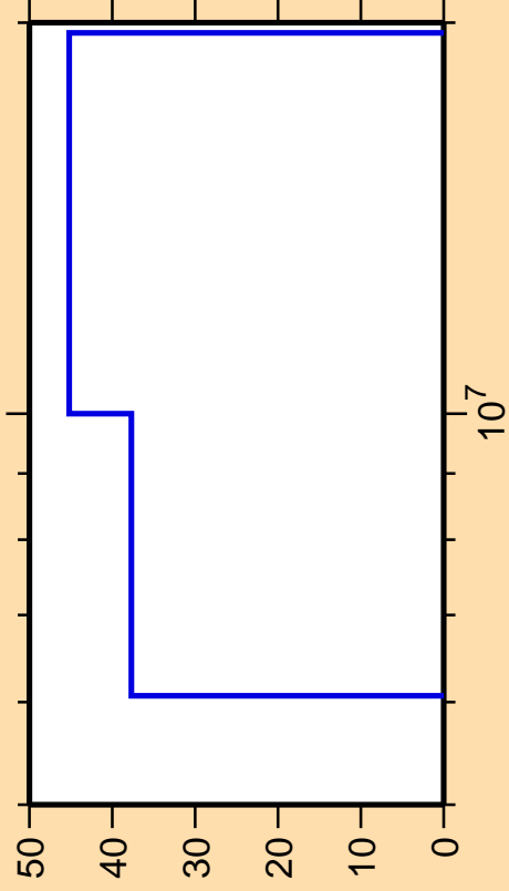
\Delta\sigma/\sigma vs. E for ^{253}\text{Es}(n,t)
