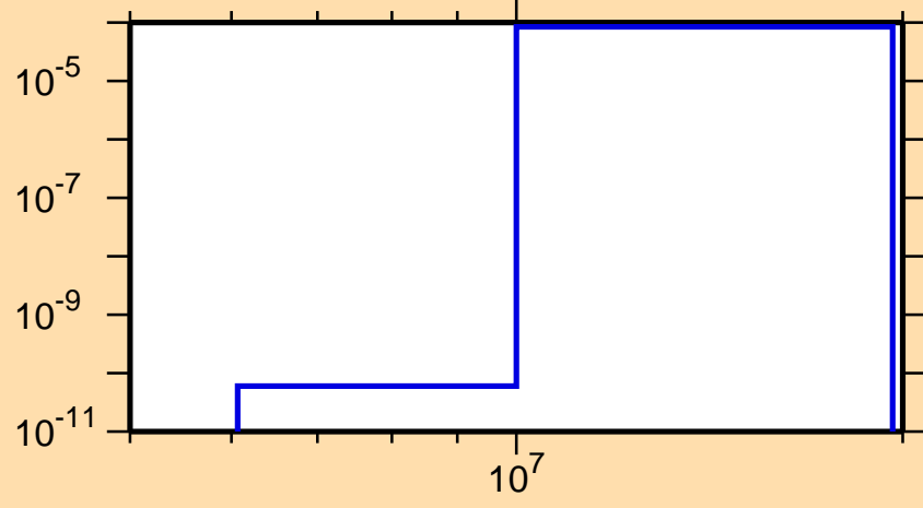
\sigma vs. E for ^{253}\text{Es}(n,t)
