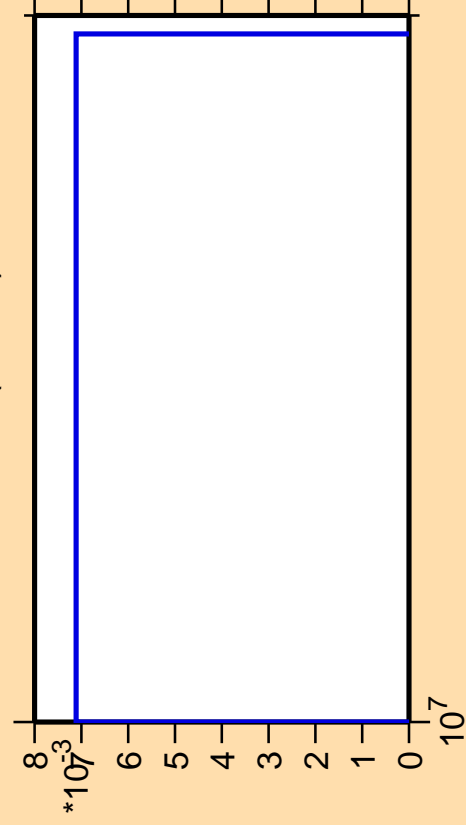
\Delta\sigma/\sigma vs. E for ^{253}\text{Es} (mt 42)
