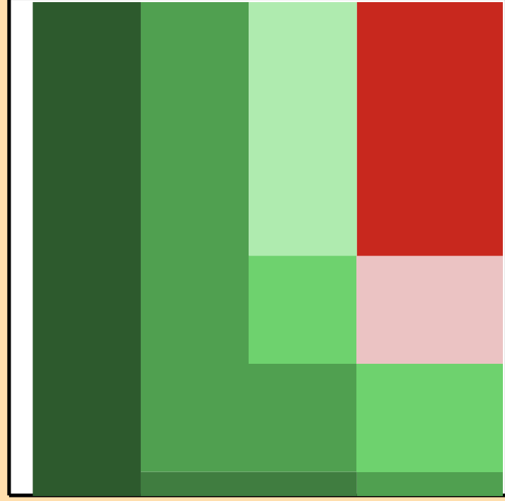
\Delta\sigma/\sigma vs. E for ^{253}\text{Es}(n,p)
