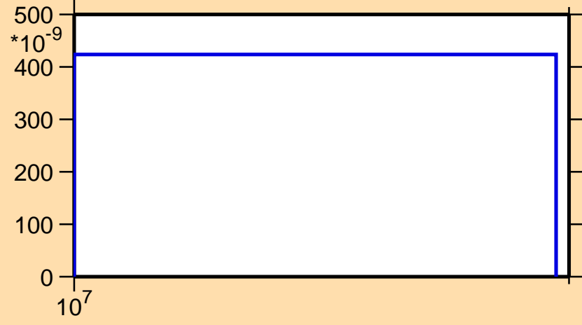
\sigma vs. E for ^{253}\text{Es}(n,nt)
