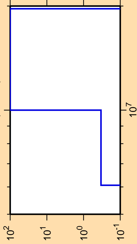
\Delta\sigma/\sigma vs. E for ^{253}\text{Es}(n,2n\alpha)
