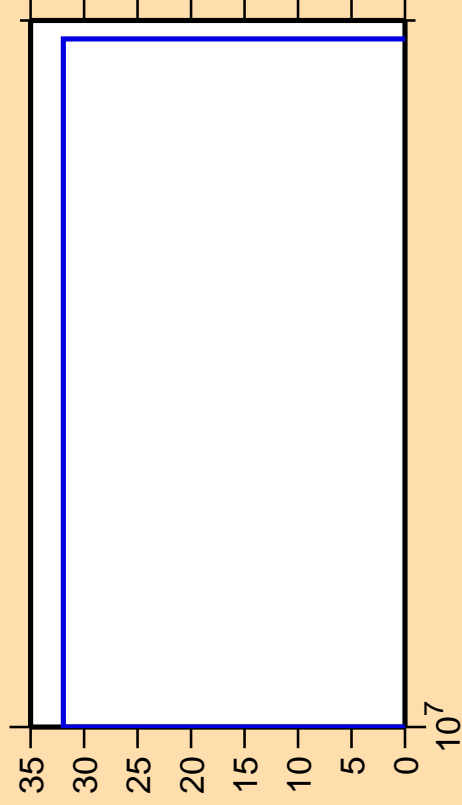
\Delta\sigma/\sigma vs. E for ^{253}\text{Es}(n,nt)
