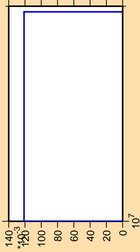
\Delta\sigma/\sigma vs. E for ^{253}\text{Es} (mt 11)
