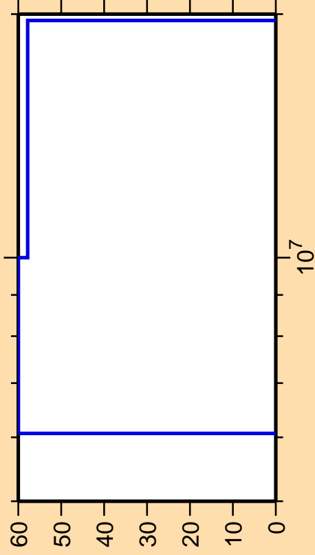
\Delta\sigma/\sigma vs. E for ^{253}\text{Es}(n,d)
