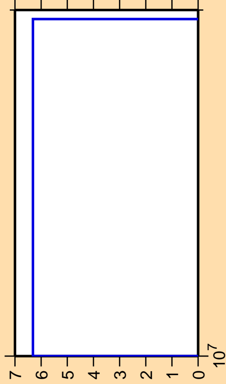
\Delta\sigma/\sigma vs. E for ^{253}\text{Es}(n,3n\alpha)
