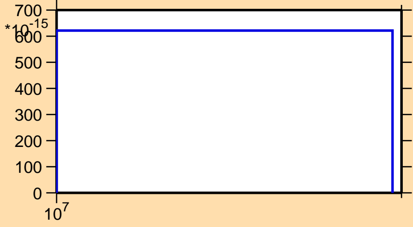
\sigma vs. E for ^{253}\text{Es}(n,\text{He}3)
