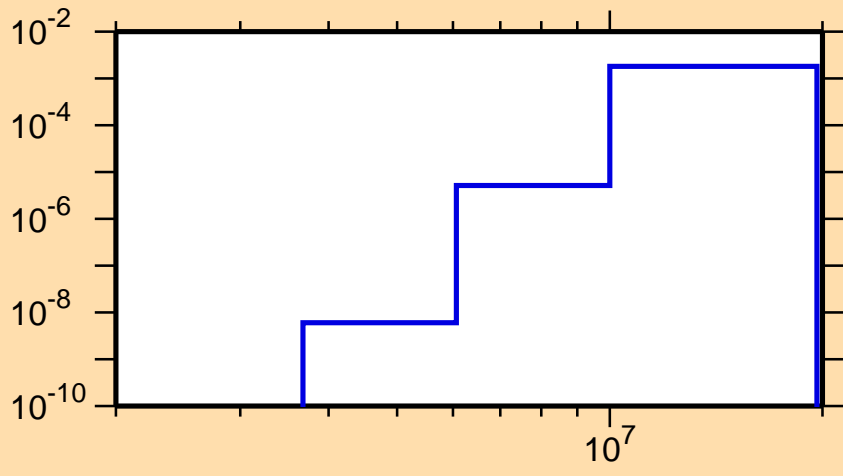
\sigma vs. E for ^{253}\text{Es}(n,p)
