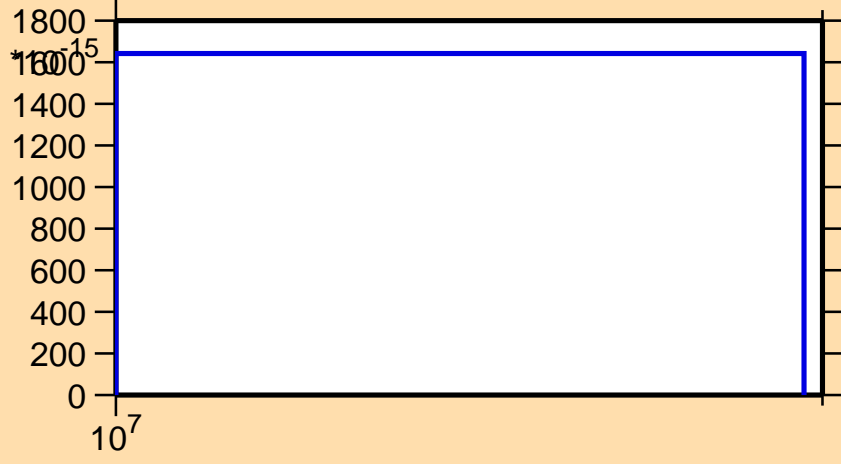
\sigma vs. E for ^{253}\text{Es}(n,3n\alpha)
