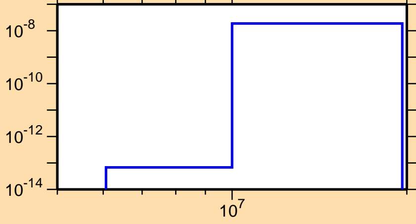
\sigma vs. E for ^{253}\text{Es}(n,2n\alpha)
