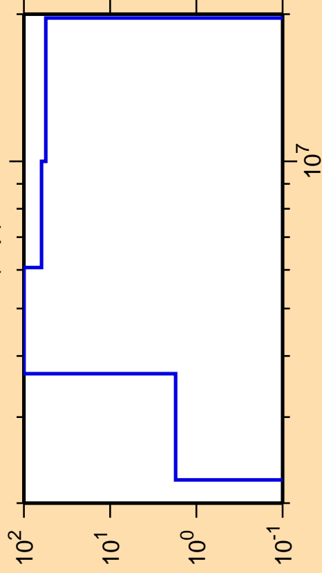
\Delta\sigma/\sigma vs. E for ^{253}\text{Es}(n,p)
