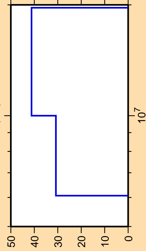
\Delta\sigma/\sigma vs. E for ^{253}\text{Es}(n,f)
