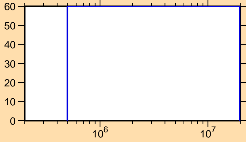
\Delta\sigma/\sigma vs. E for ^{253}\text{Es}(n,n\text{cont.})
