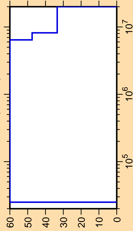
\Delta\sigma/\sigma vs. E for ^{253}\text{Es}(n,\text{inel.})
