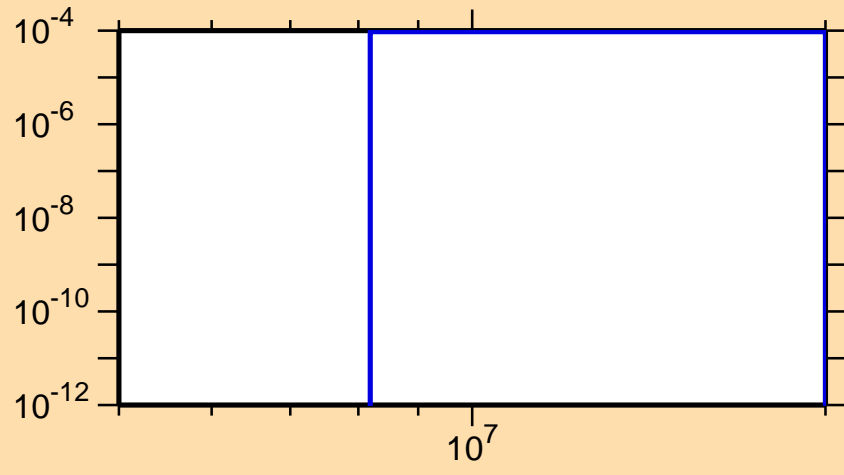
\sigma vs. E for ^{253}\text{Es}(n,np)
