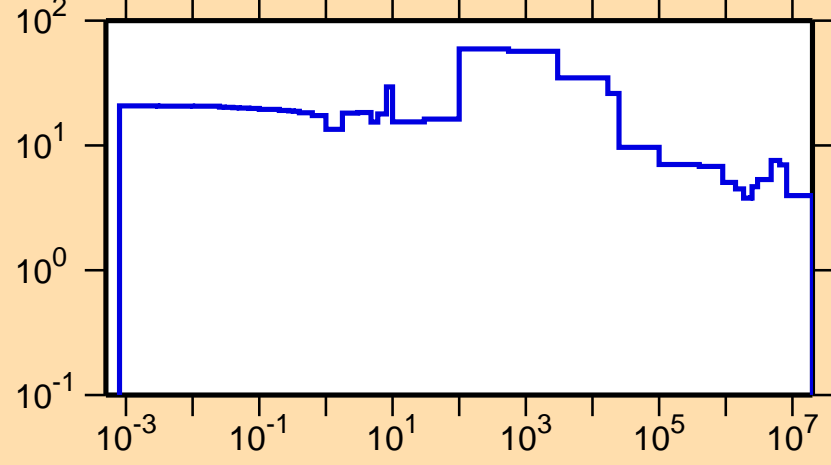
\Delta\sigma/\sigma vs. E for ^{253}\text{Es}(n,\text{tot.})
