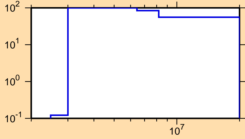
\Delta\sigma/\sigma vs. E for ^{253}\text{Es}(n,p)
