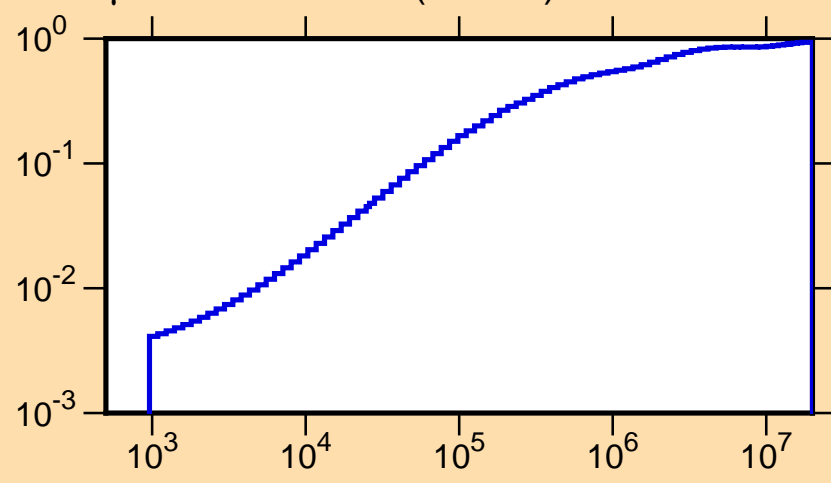
\mu vs. E for ^{254}\text{Es}(\text{mt251})
