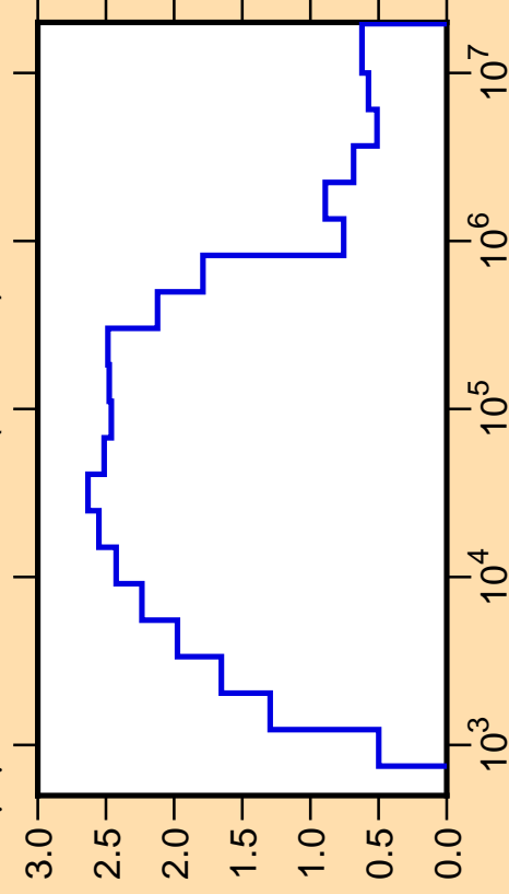
\Delta\mu/\mu vs. E for ^{254}\text{Es}(\text{mt251})
