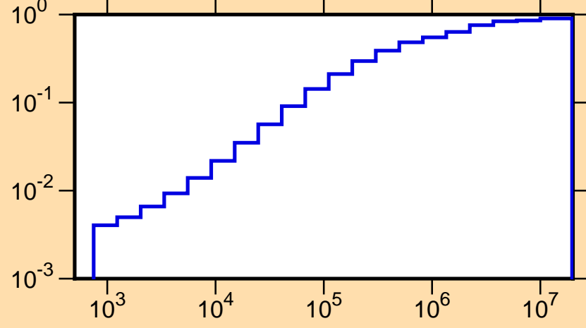
\mu vs. E for ^{254}\text{Es}(\text{mt251})
