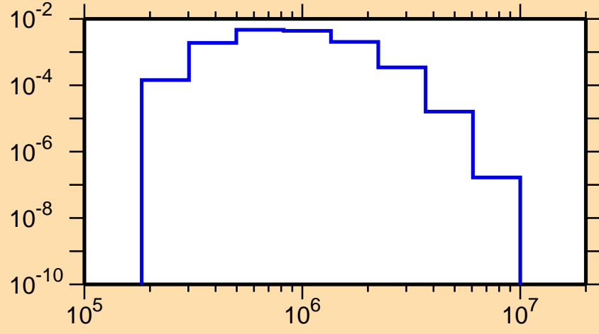
\sigma vs. E for ^{254}\text{Es}(n,n_4)
