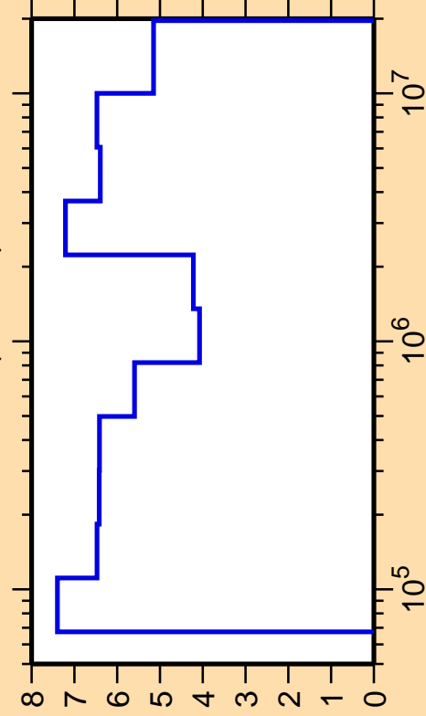
\Delta\sigma/\sigma vs. E for ^{254}\text{Es}(n,\text{inel.})
