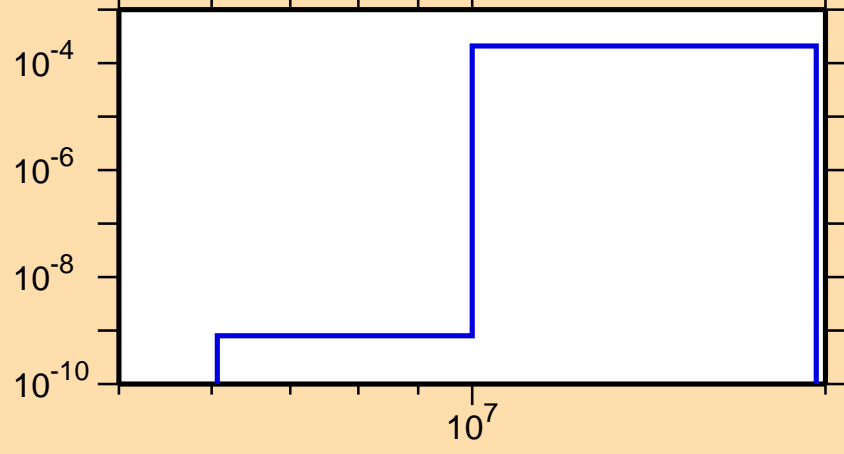
\sigma vs. E for ^{254}\text{Es}(n,d)
