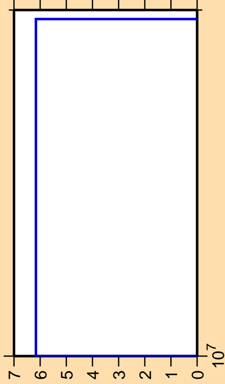
\Delta\sigma/\sigma vs. E for ^{254}\text{Es}(n,3n\alpha)
