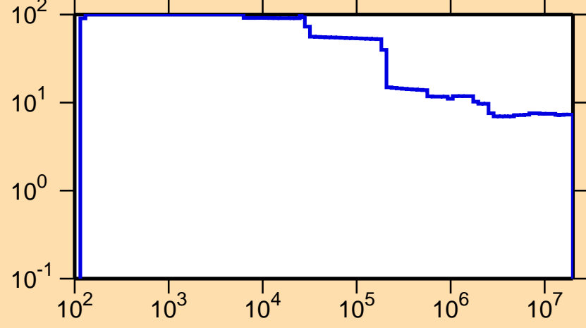
\Delta\sigma/\sigma vs. E for ^{254}\text{Es}(n,\text{nonel.})
