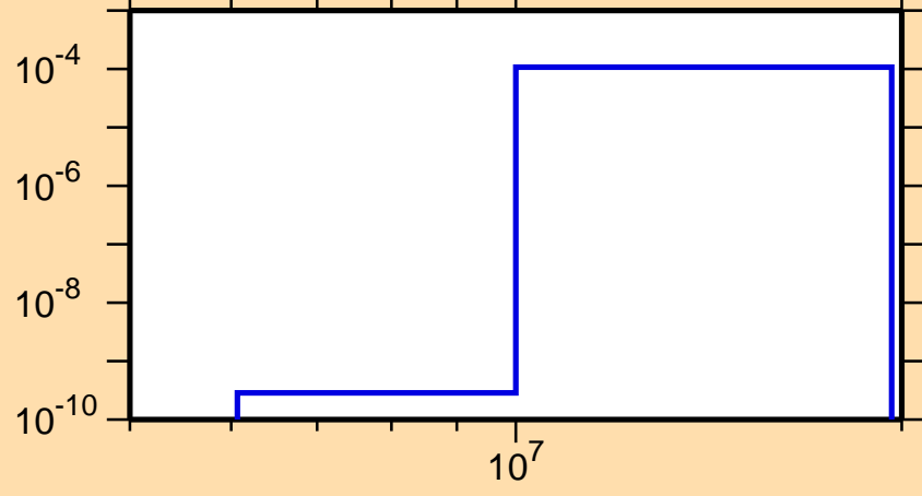
\sigma vs. E for ^{254}\text{Es}(n,np)
