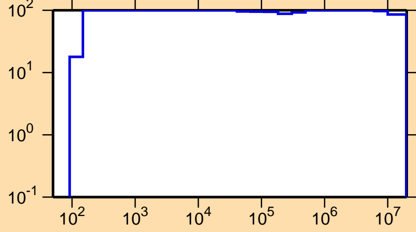
\Delta\sigma/\sigma vs. E for ^{254}\text{Es}(n,f)
