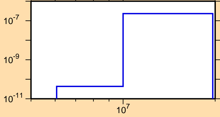
\sigma vs. E for ^{254}\text{Es}(n,2n\alpha)
