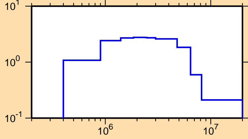
\sigma vs. E for ^{254}\text{Es}(n,n\text{cont.})
