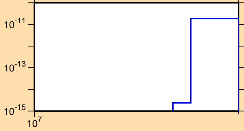
\sigma vs. E for ^{255}\text{Es} (mt 11)
