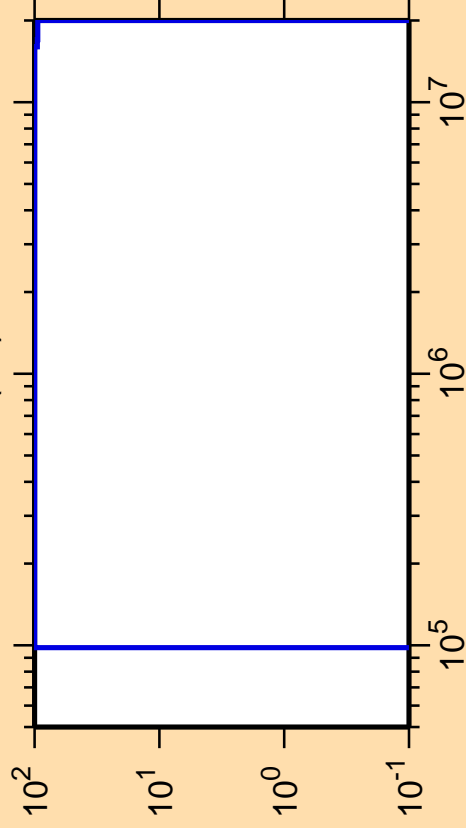
\Delta\sigma/\sigma vs. E for ^{255}\text{Es}(n,f)
