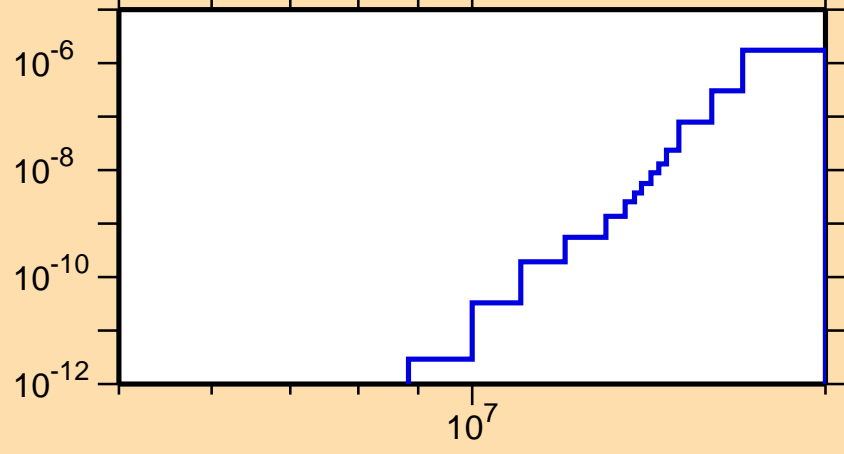
\sigma vs. E for ^{255}\text{Es}(n,2n\alpha)
