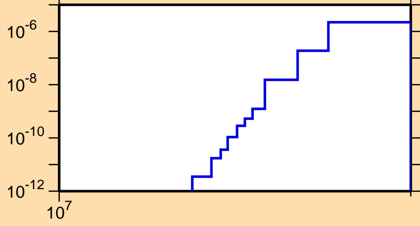
\sigma vs. E for ^{255}\text{Es}(n,nd)
