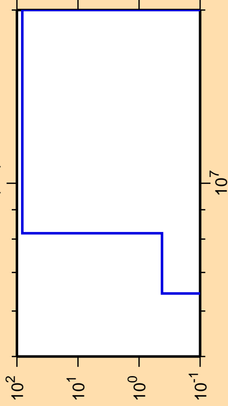
\Delta\sigma/\sigma vs. E for ^{255}\text{Es}(n,t)
