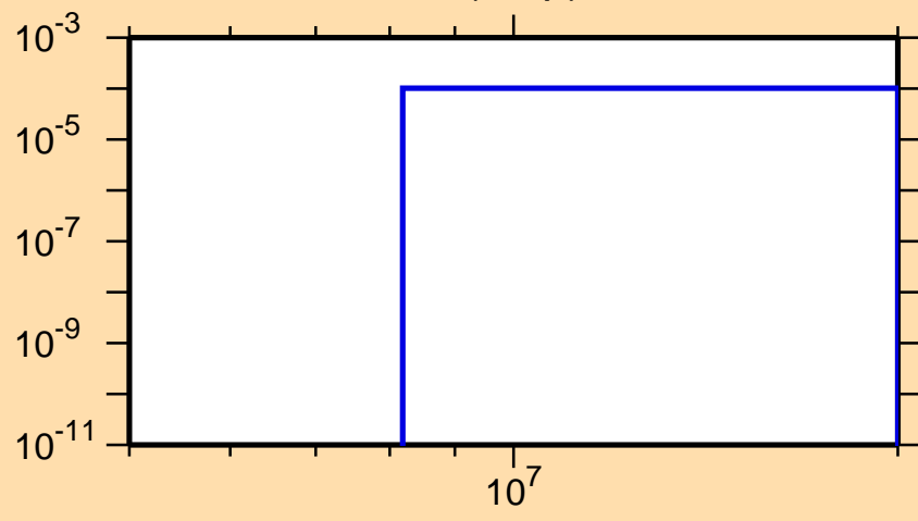
\sigma vs. E for ^{255}\text{Es}(n,np)
