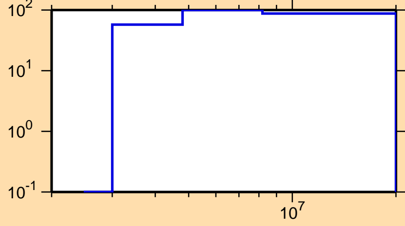
\Delta\sigma/\sigma vs. E for ^{255}\text{Es}(n,p)
