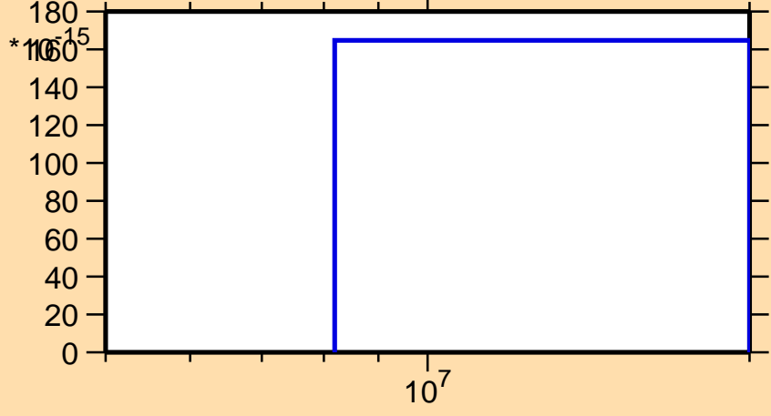
\sigma vs. E for ^{255}\text{Es}(n,\text{He}3)
