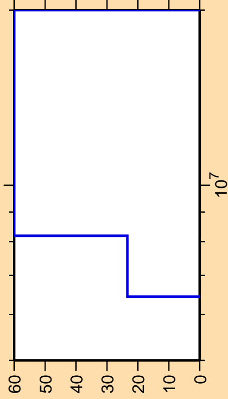
\Delta\sigma/\sigma vs. E for ^{255}\text{Es}(n,d)
