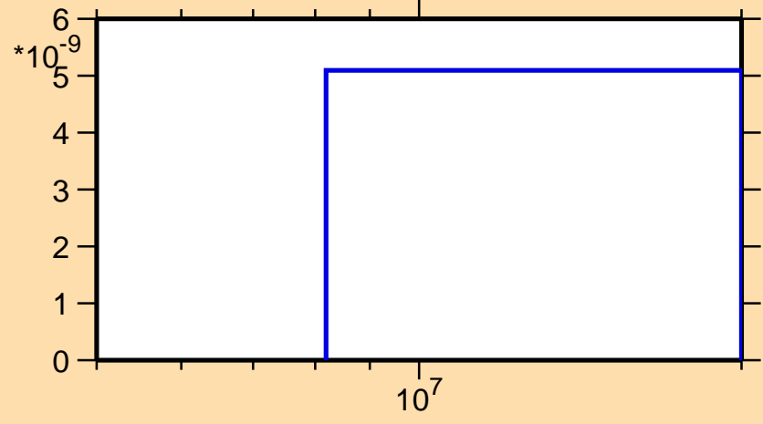
\sigma vs. E for ^{255}\text{Es}(n,2np)
