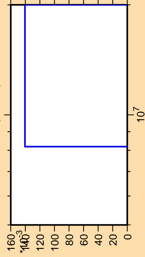
\Delta\sigma/\sigma vs. E for ^{255}\text{Es} (mt 11)
