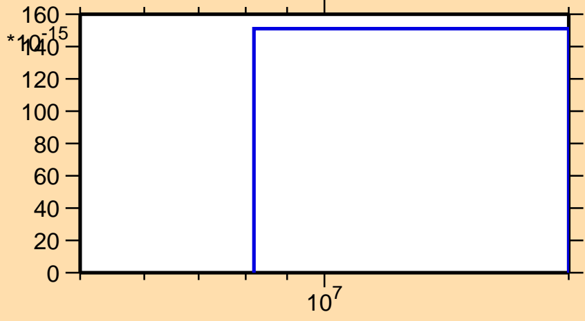
\sigma vs. E for ^{255}\text{Es} (mt 11)
