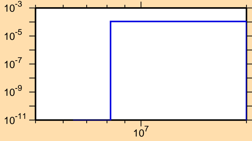
\sigma vs. E for ^{255}\text{Es}(n,d)
