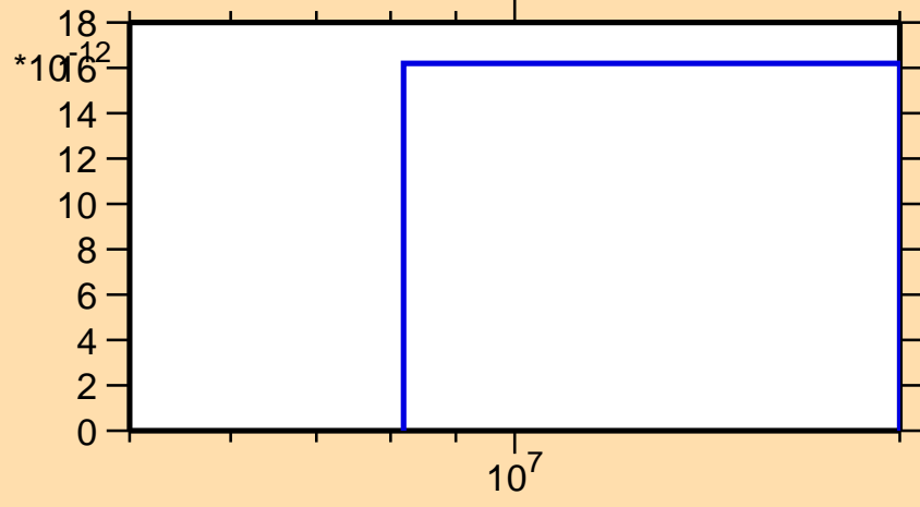
\sigma vs. E for ^{255}\text{Es}(n,3n\alpha)
