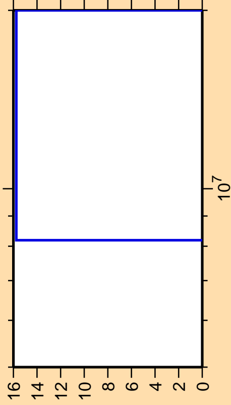
\Delta\sigma/\sigma vs. E for ^{255}\text{Es}(n,3n\alpha)
