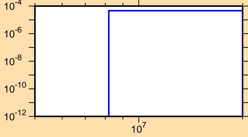
\sigma vs. E for ^{255}\text{Es}(n,t)
