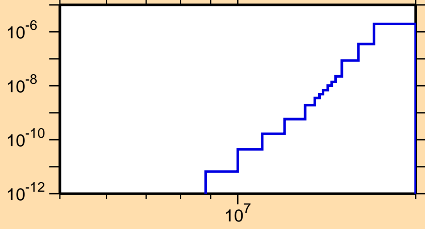
\sigma vs. E for ^{256}\text{Es}(n,2n\alpha)
