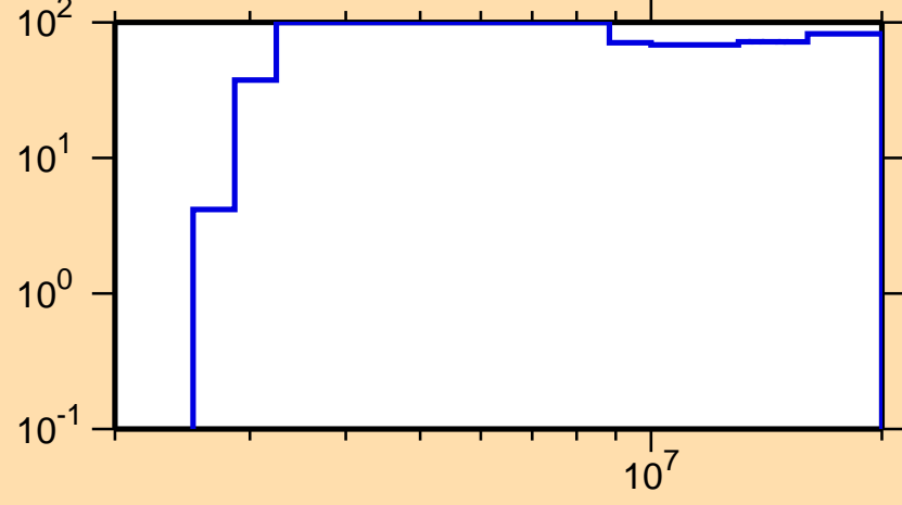
\Delta\sigma/\sigma vs. E for ^{256}\text{Es}(n,p)
