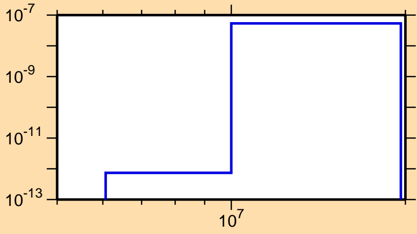
\sigma vs. E for ^{256}\text{Es}(n,2n\alpha)
