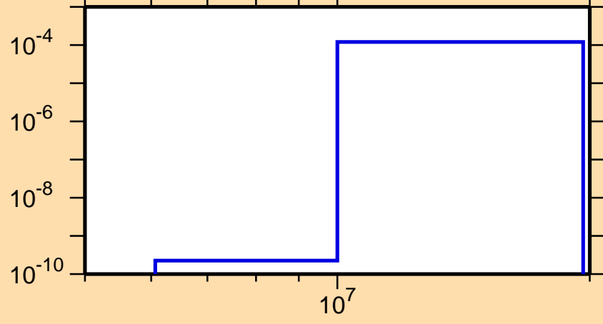
\sigma vs. E for ^{256}\text{Es}(n,d)
