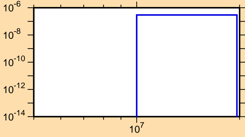
\sigma vs. E for ^{256}\text{Es}(n,nt)
