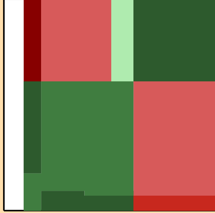
\Delta\sigma/\sigma vs. E for ^{256}\text{Es}(n,p)
