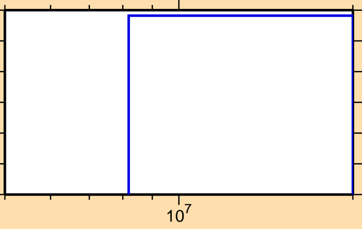
\sigma vs. E for ^{256}\text{Es}(n,3n)
