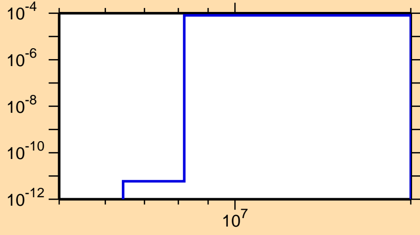
\sigma vs. E for ^{256}\text{Es}(n,t)
