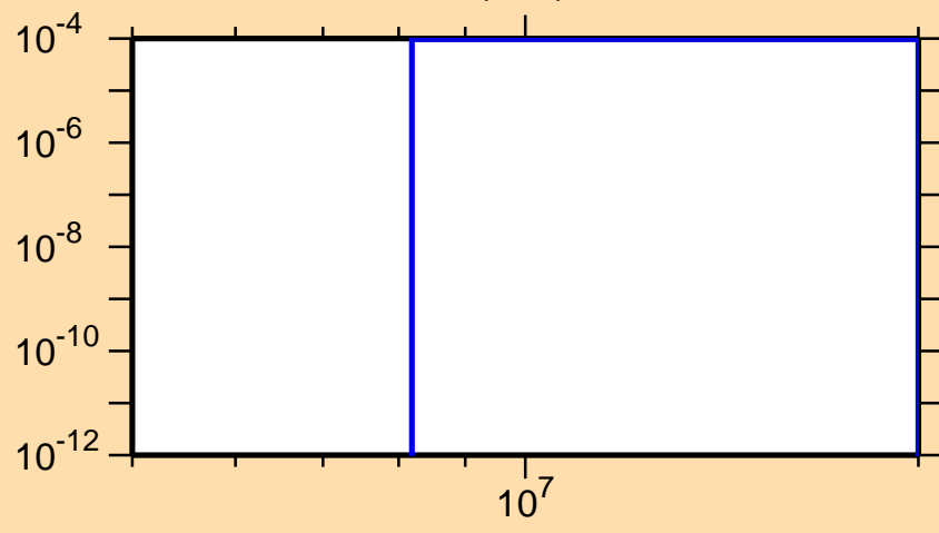
\sigma vs. E for ^{256}\text{Es}(n,d)
