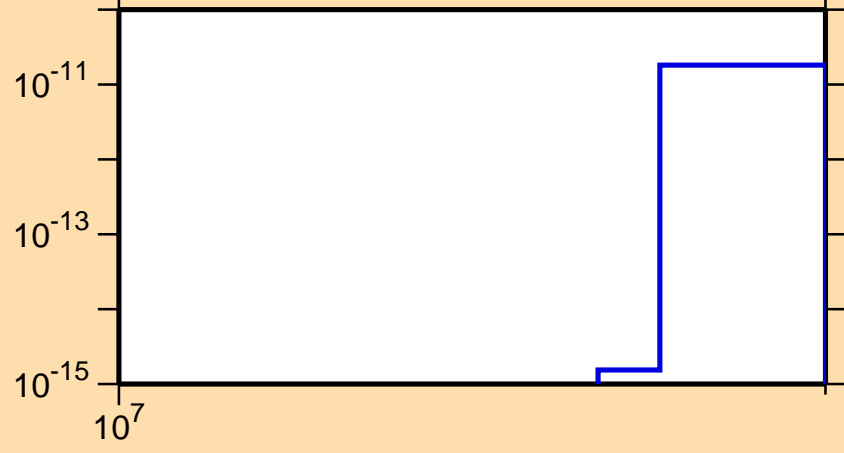
\sigma vs. E for ^{256}\text{Es} (mt 11)
