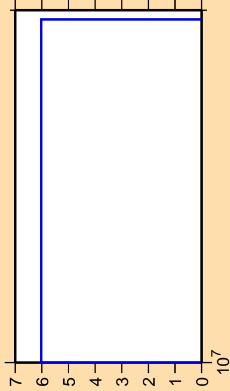
\Delta\sigma/\sigma vs. E for ^{256}\text{Es}(n,3n\alpha)
