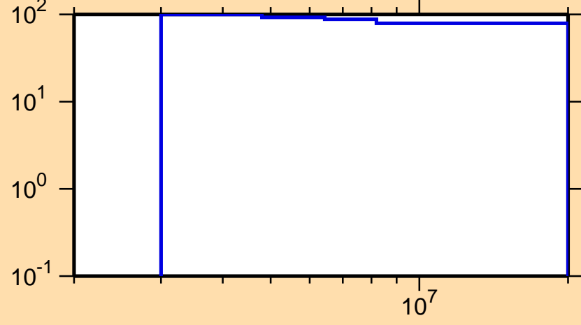
\Delta\sigma/\sigma vs. E for ^{256}\text{Es}(n,2n)
