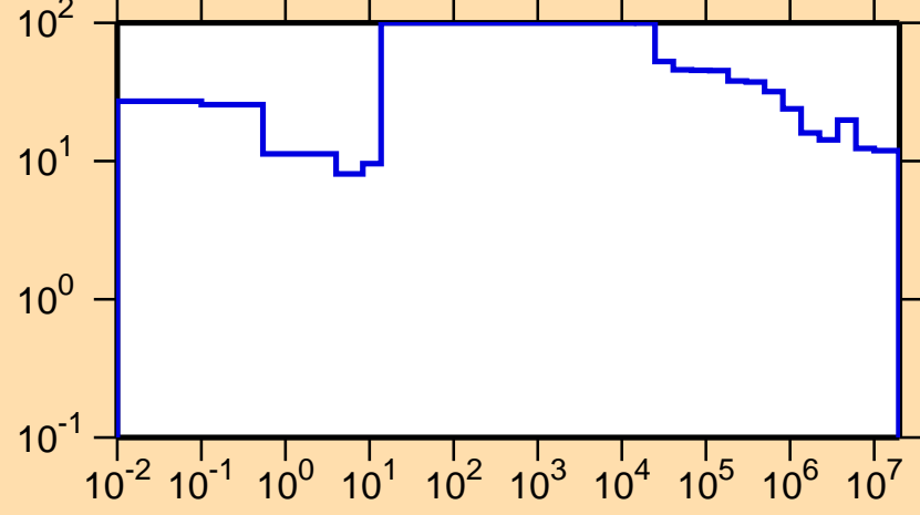
\Delta\sigma/\sigma vs. E for ^{257}\text{Es}(n,\text{tot.})
