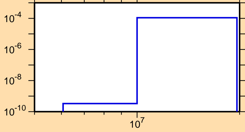
\sigma vs. E for ^{257}\text{Es}(n,d)
