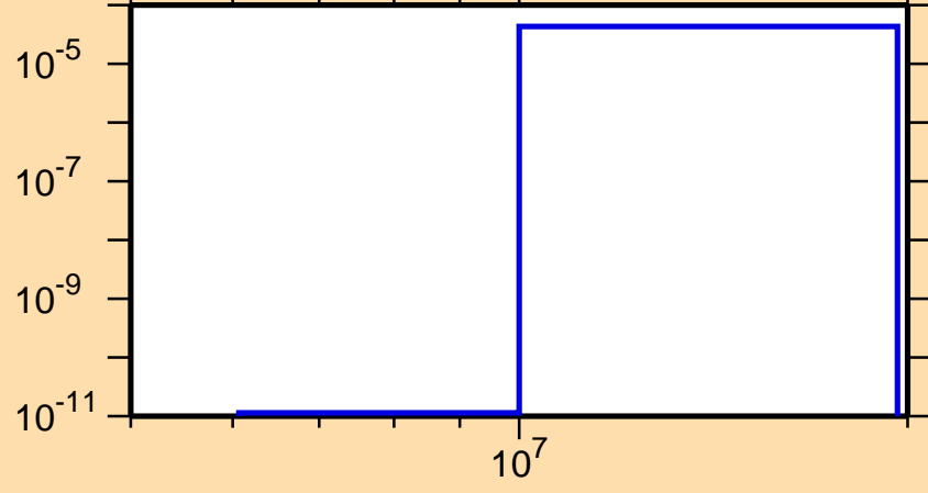
\sigma vs. E for ^{257}\text{Es}(n,t)
