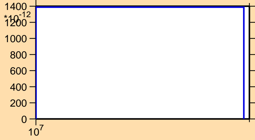
\sigma vs. E for ^{257}\text{Es}(n,2np)
