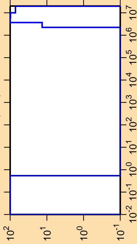
\Delta\sigma/\sigma vs. E for ^{257}\text{Es}(n,\alpha)
