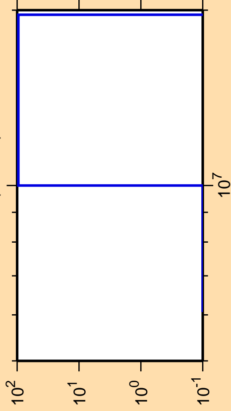
\Delta\sigma/\sigma vs. E for ^{257}\text{Es}(n,2n\alpha)
