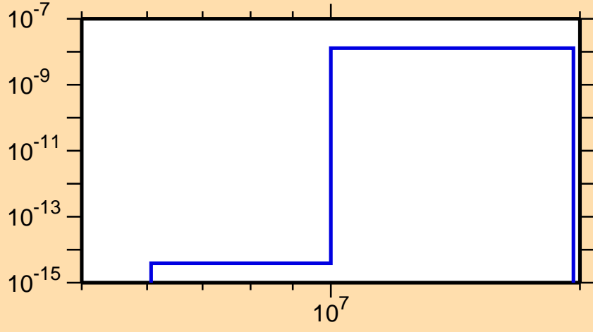
\sigma vs. E for ^{257}\text{Es}(n,2n\alpha)
