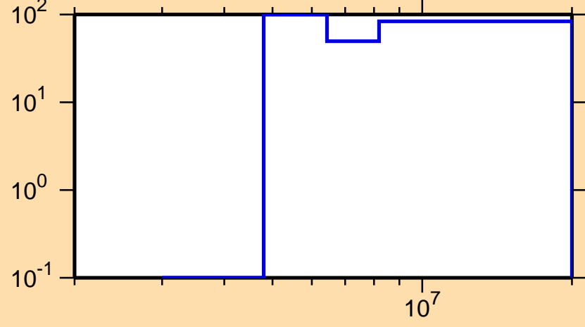
\Delta\sigma/\sigma vs. E for ^{257}\text{Es}(n,p)
