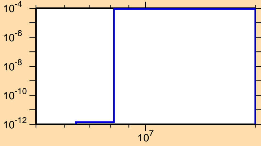
\sigma vs. E for ^{257}\text{Es}(n,d)
