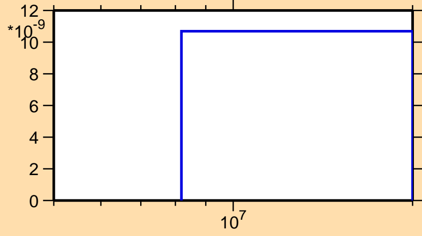
\sigma vs. E for ^{257}\text{Es}(n,2n\alpha)
