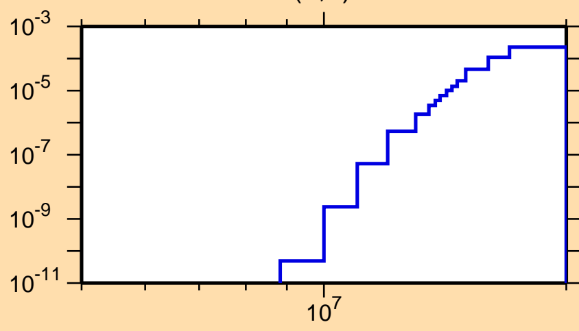
\sigma vs. E for ^{258}\text{Es}(n,d)
