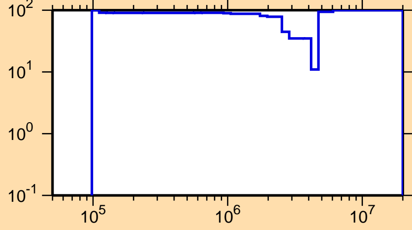
\Delta\sigma/\sigma vs. E for ^{258}\text{Es}(n,\text{inel.})
