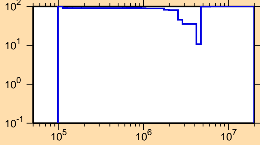
\Delta\sigma/\sigma vs. E for ^{258}\text{Es}(n,n\text{cont.})
