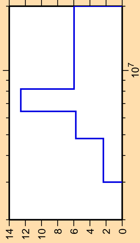
\Delta\sigma/\sigma vs. E for ^{258}\text{Es}(n,n_1)
