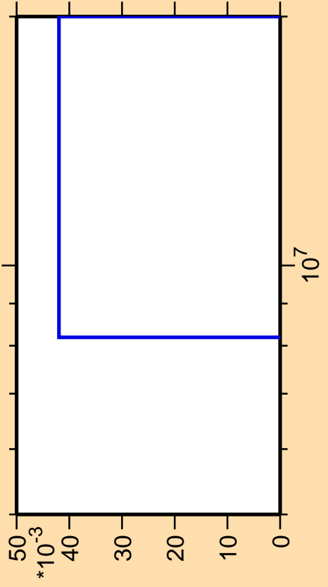
\Delta\sigma/\sigma vs. E for ^{258}\text{Es}(n,\text{He3})
