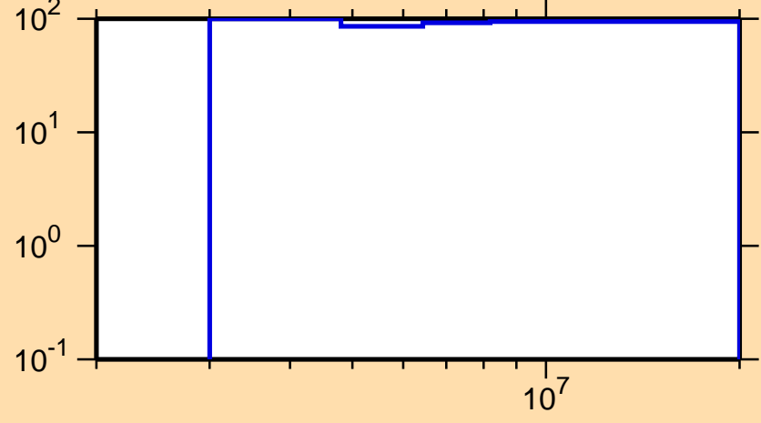
\Delta\sigma/\sigma vs. E for ^{258}\text{Es}(n,2n)
