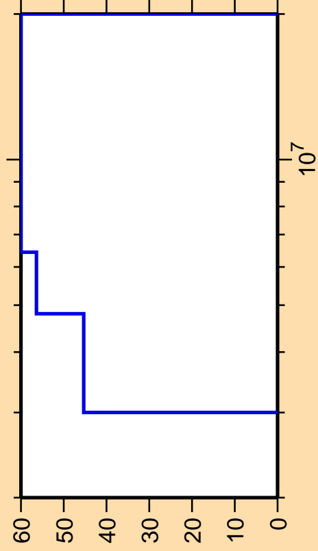
\Delta\sigma/\sigma vs. E for ^{258}\text{Es}(n,\gamma)
