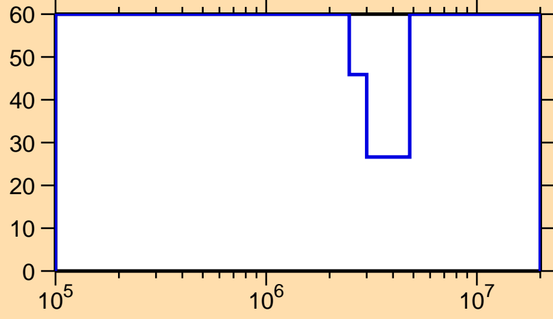
\Delta\sigma/\sigma vs. E for ^{258}\text{Es}(n,\text{inel.})
