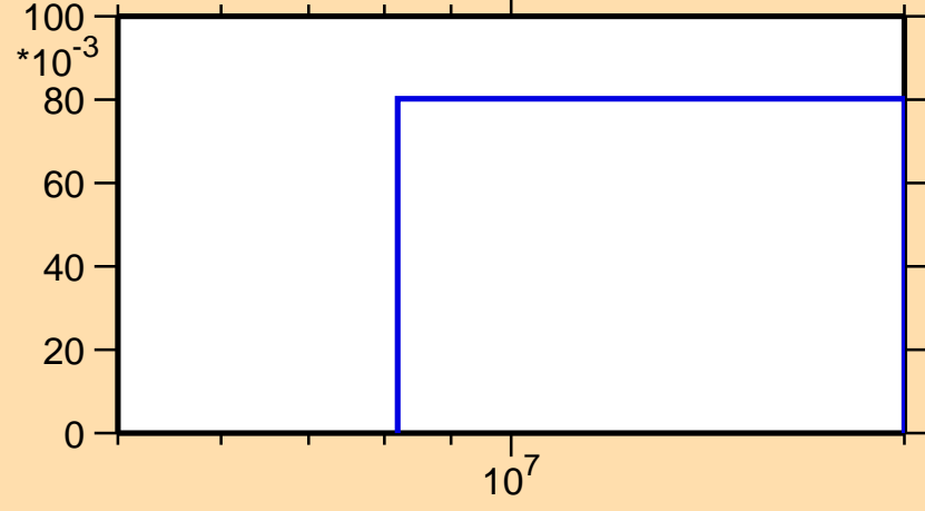
\sigma vs. E for ^{258}\text{Es}(n,3n)
