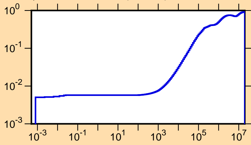
\mu vs. E for ^{135}\text{Eu}(\text{mt251})
