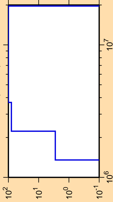
\Delta\sigma/\sigma vs. E for ^{135}\text{Eu}(n,\text{He3})
