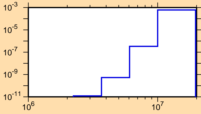
\sigma vs. E for ^{135}\text{Eu}(n,\text{He3})
